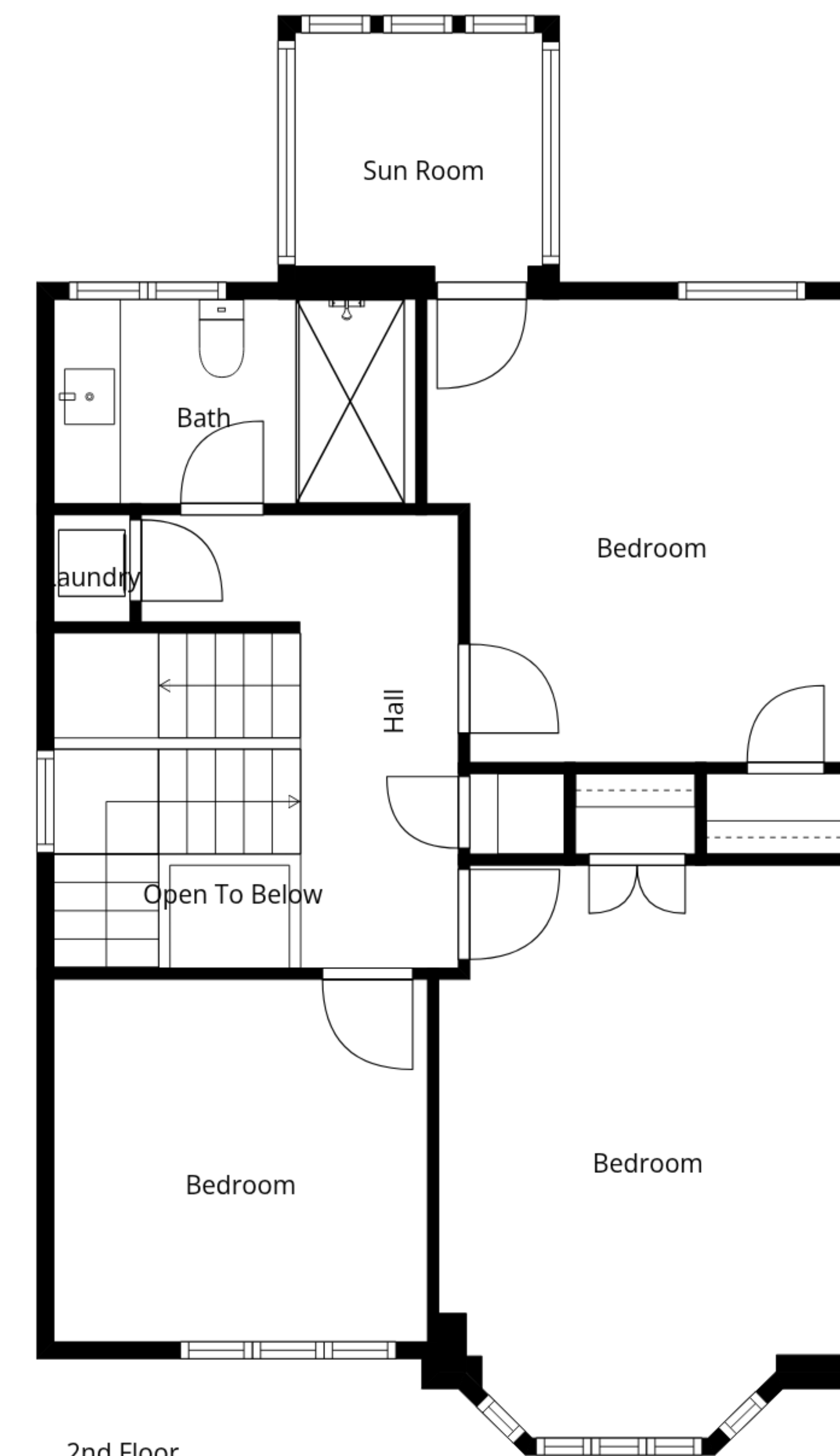
2nd Floor
