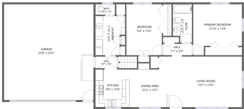
1st floor
