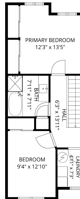
ABOVE MAIN
