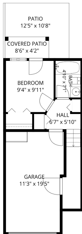
BELOW MAIN
