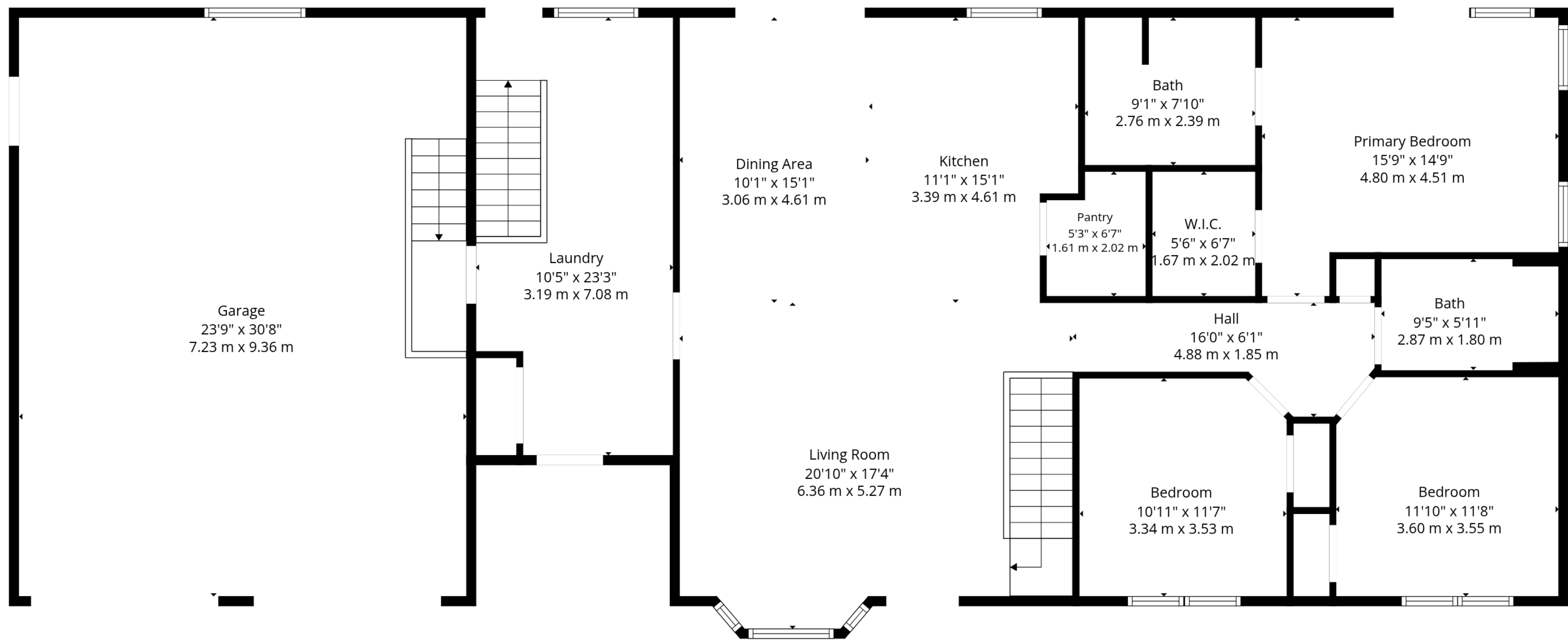
1st Floor
