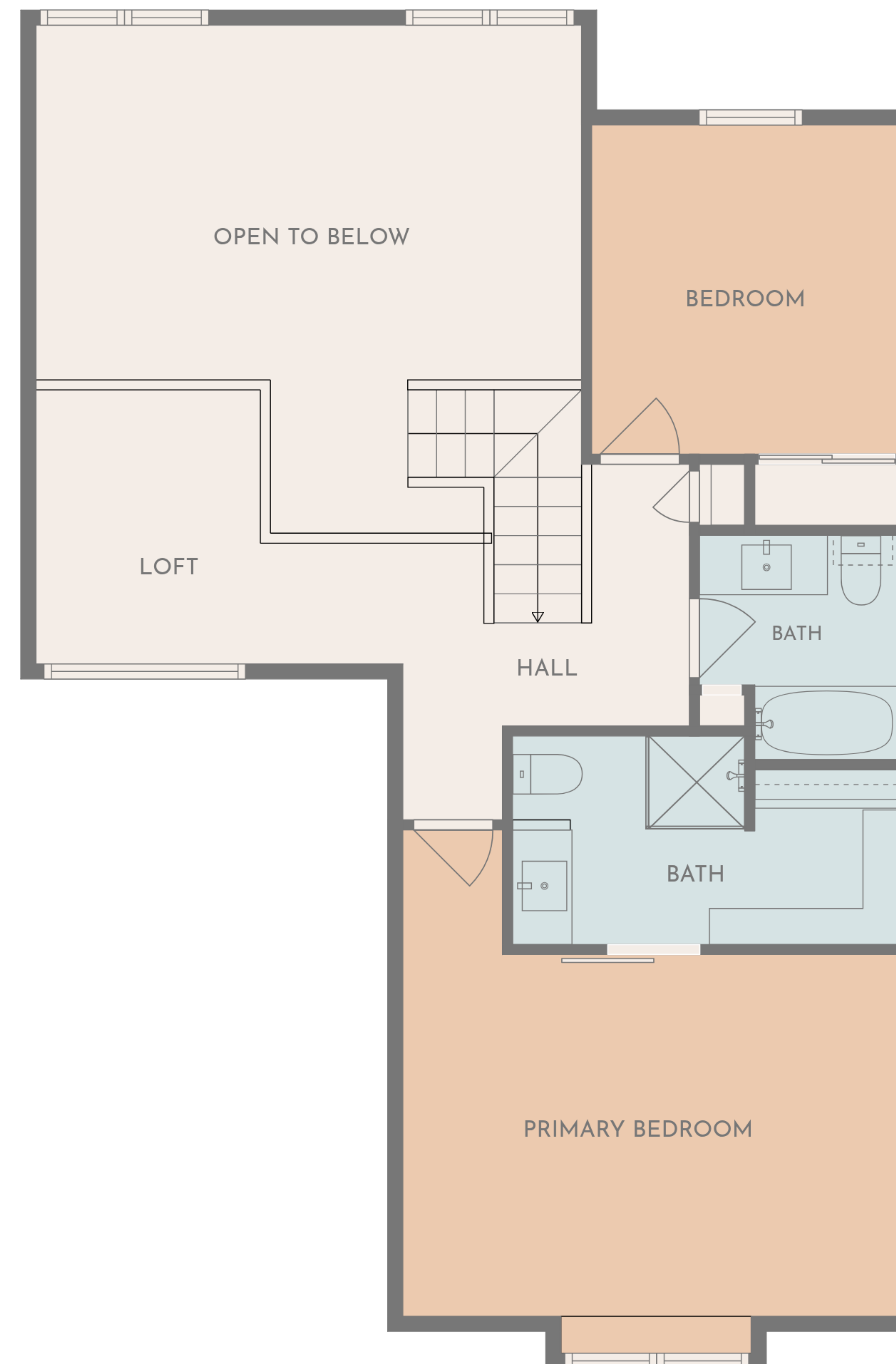
2nd floor
