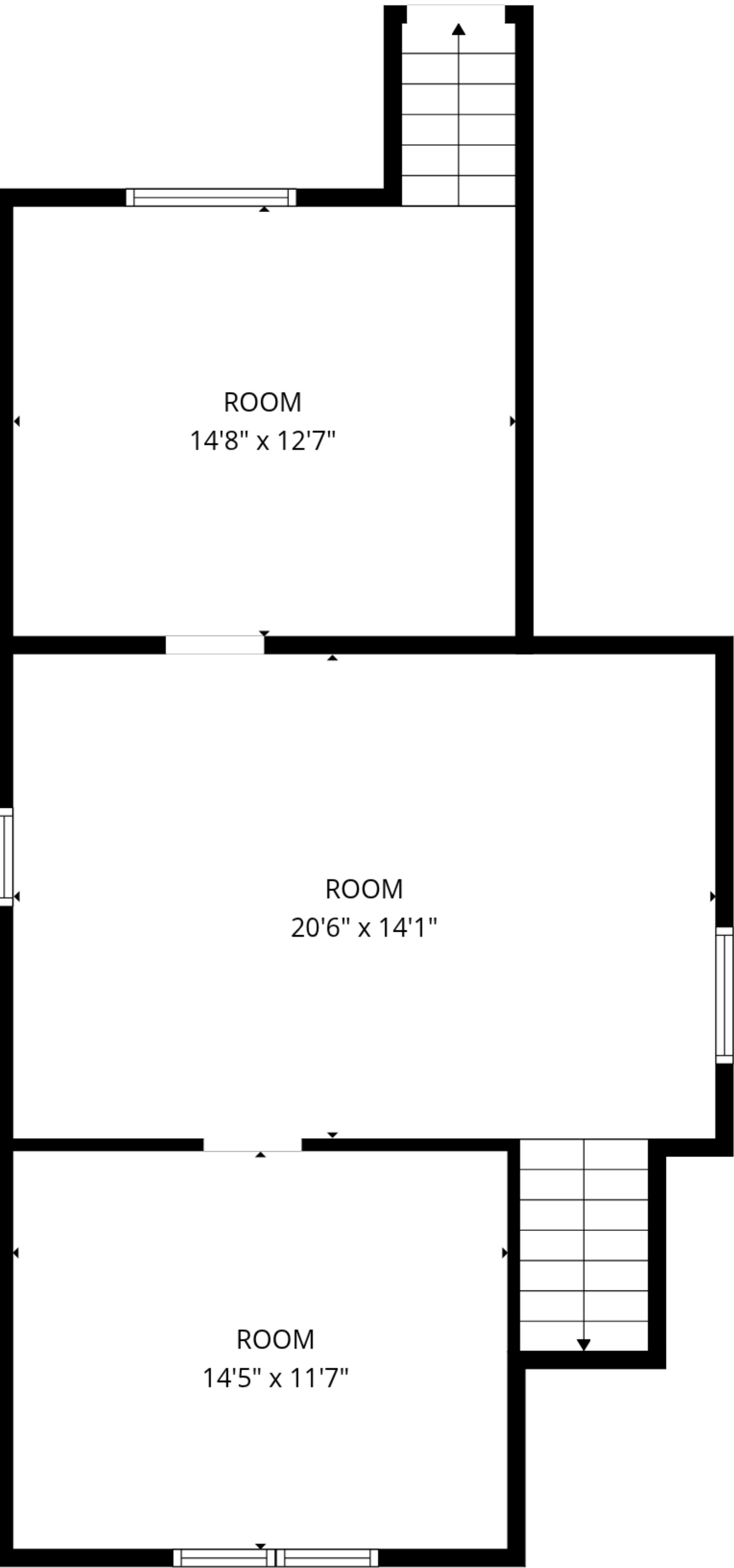
1st floor
