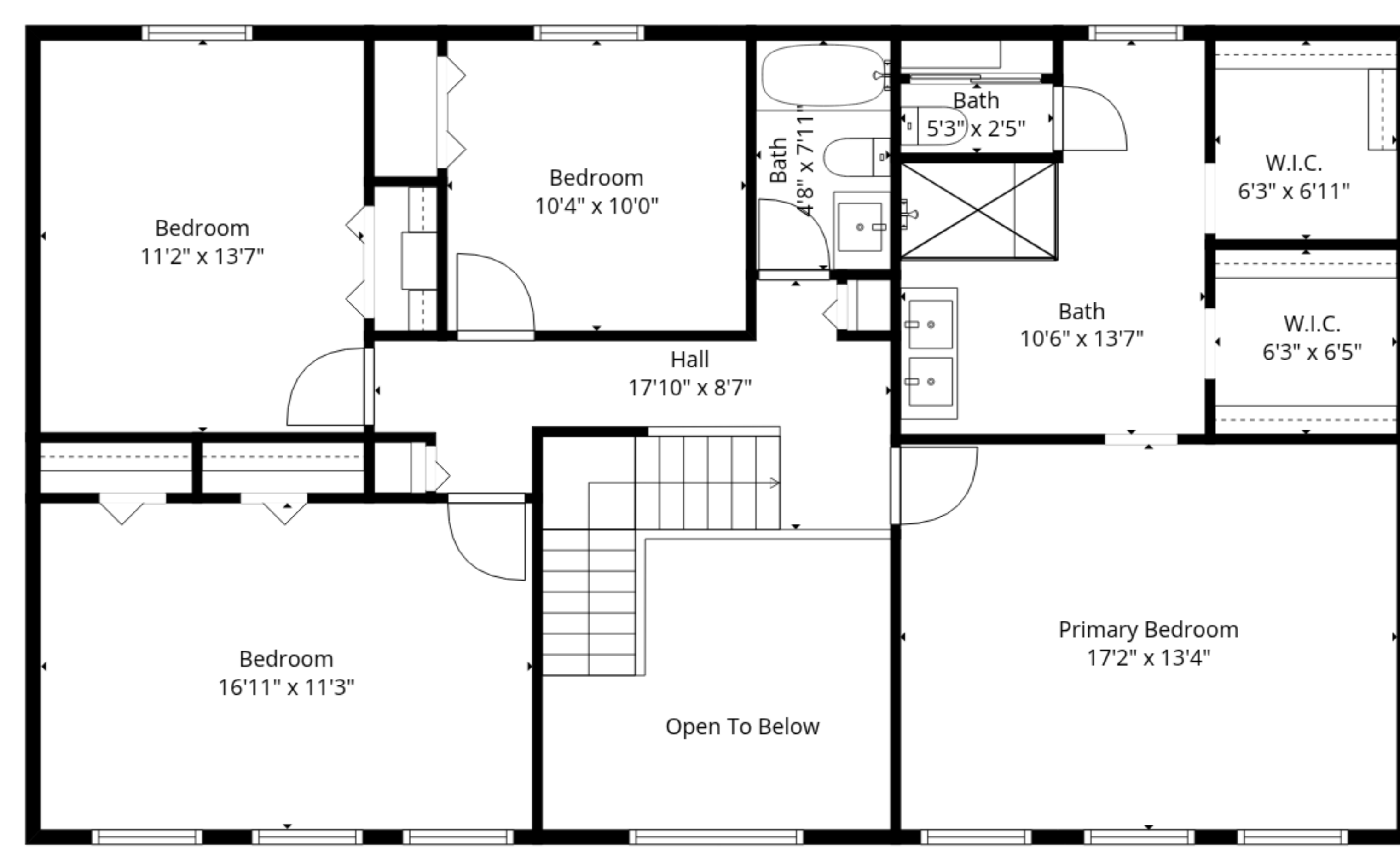
2nd Floor
