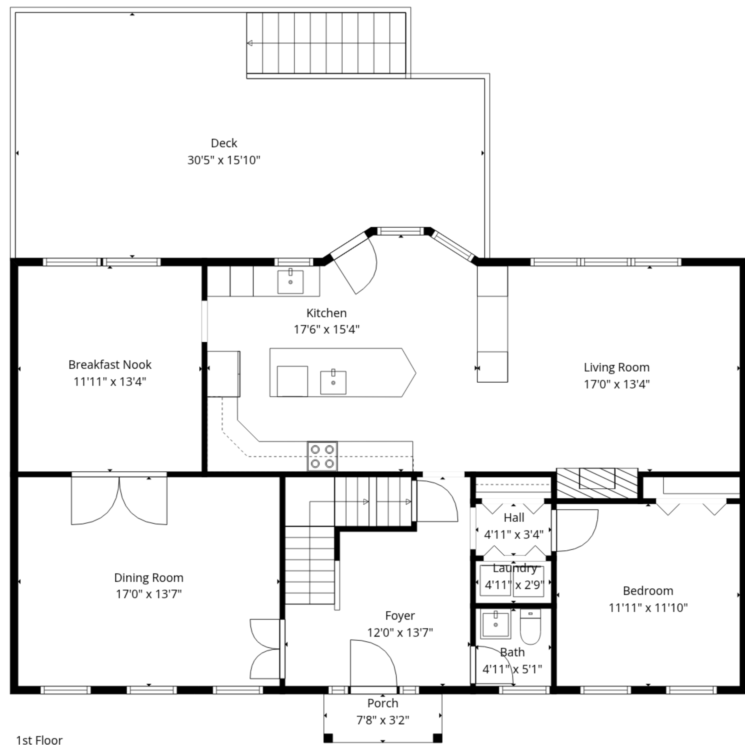
1st Floor
