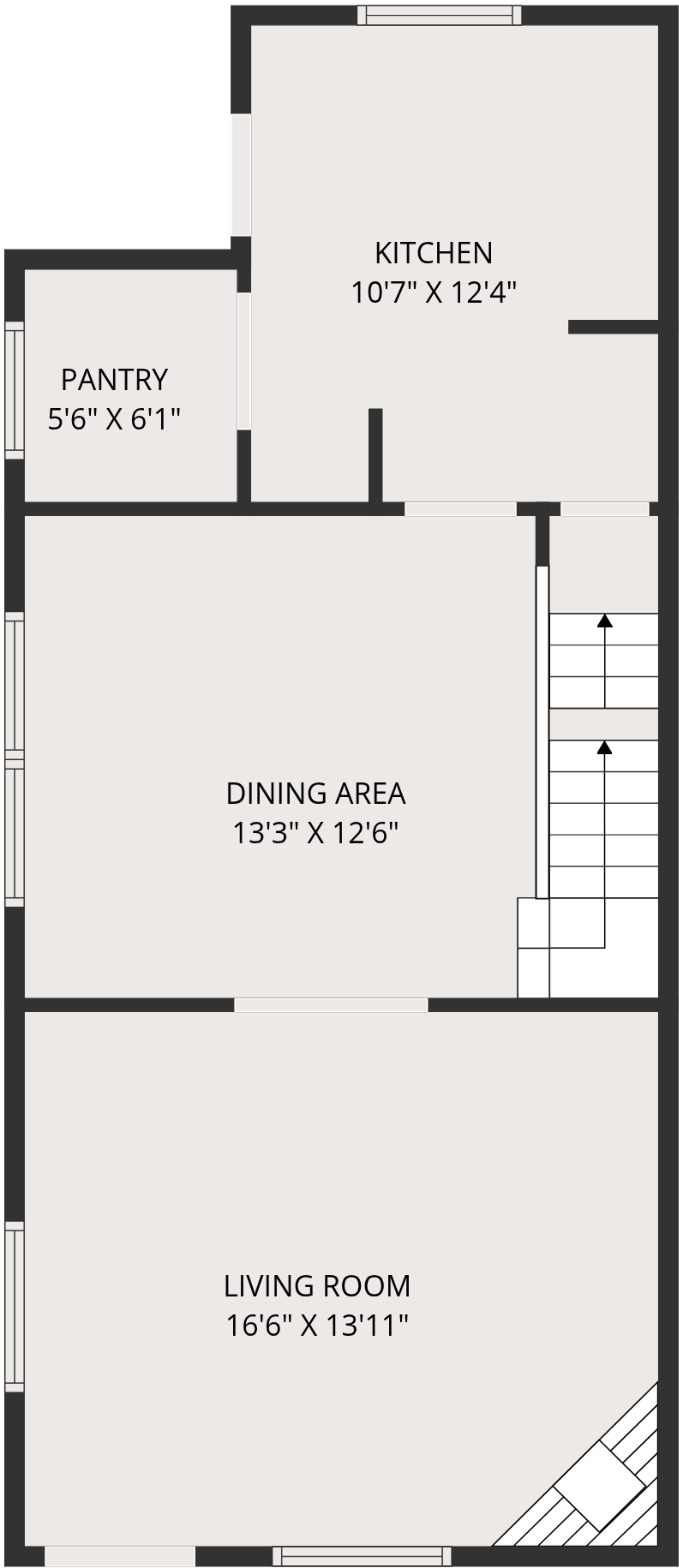
1ST FLOOR
