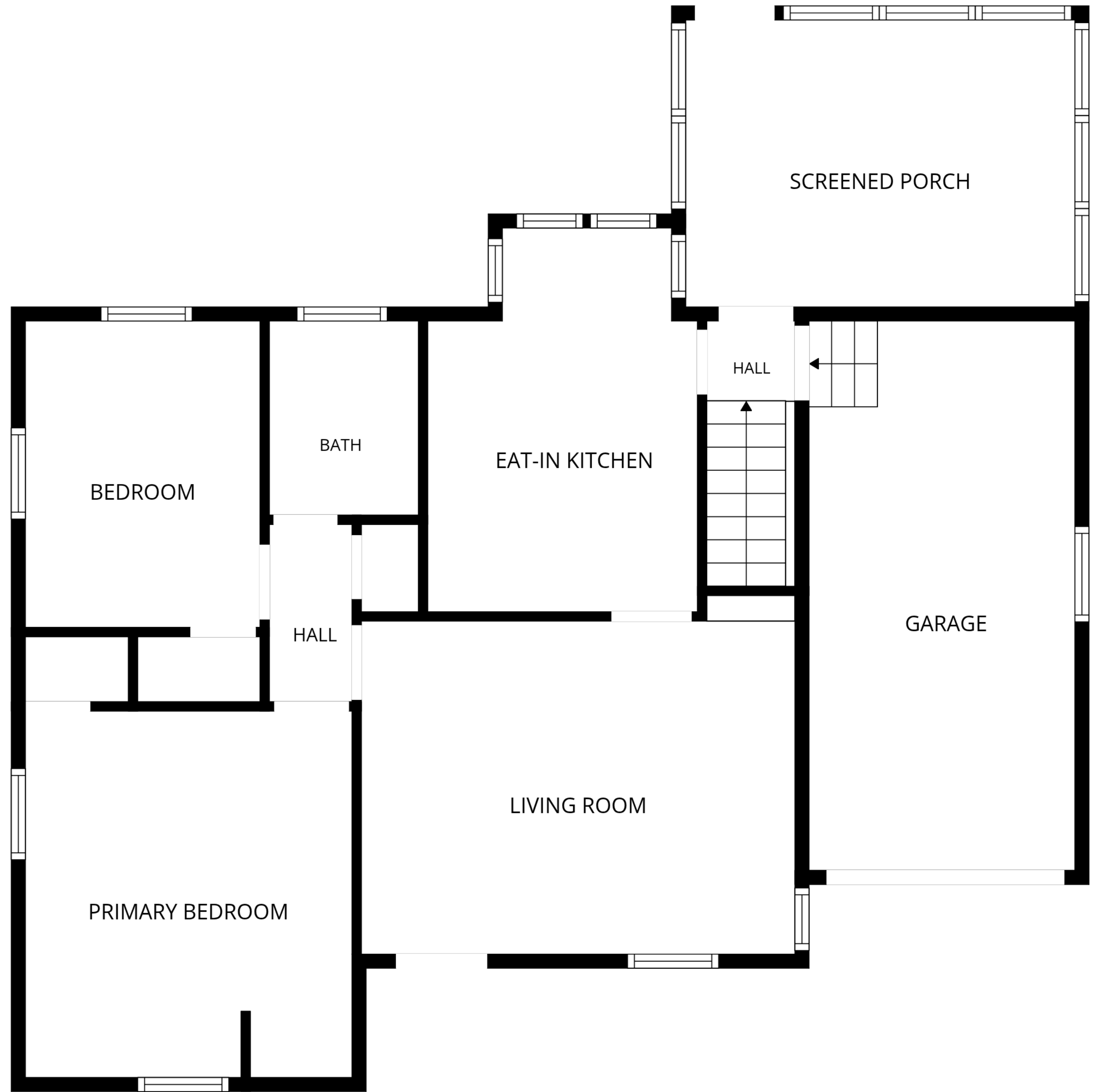
1st floor
