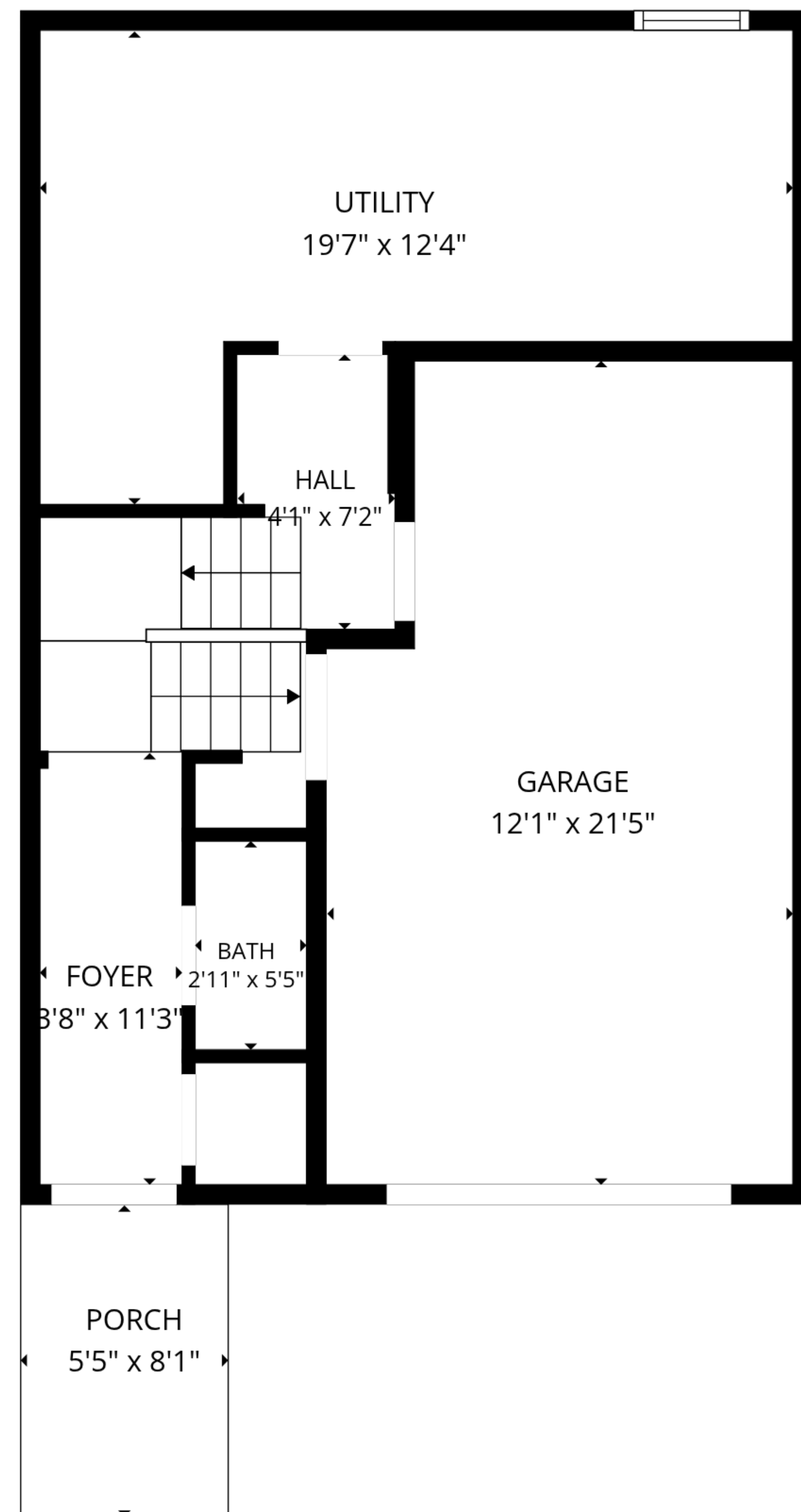
Basement
