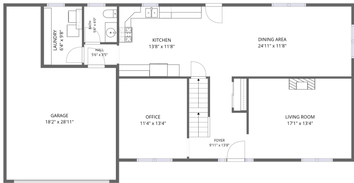
1st floor
