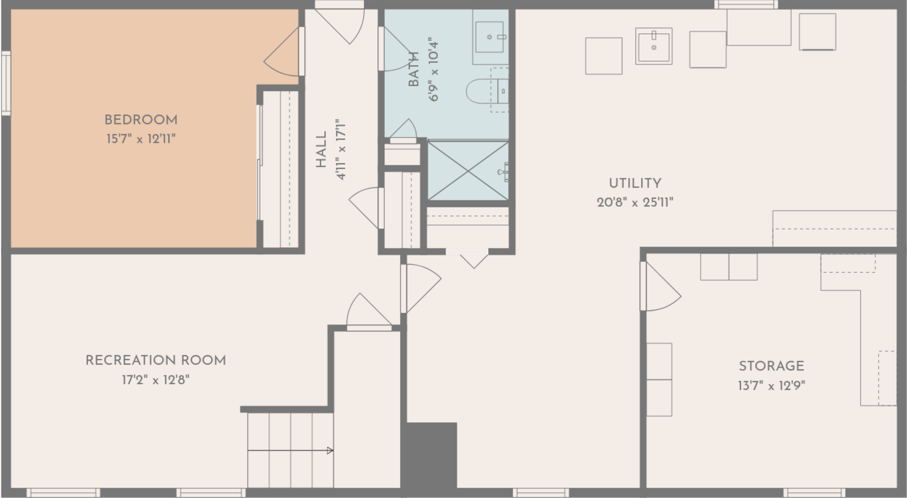
Basement
