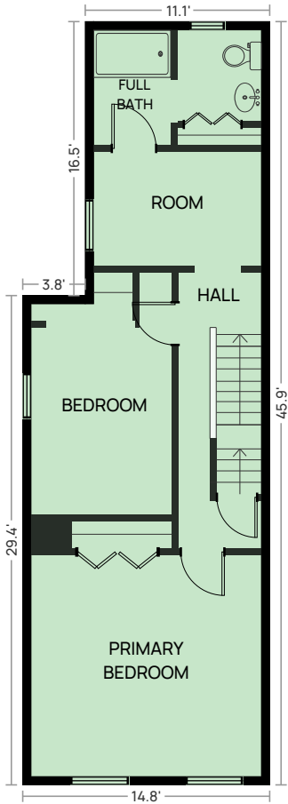
SECOND FLOOR Above grade - 8'11" ceiling GLA 620 sq ft
