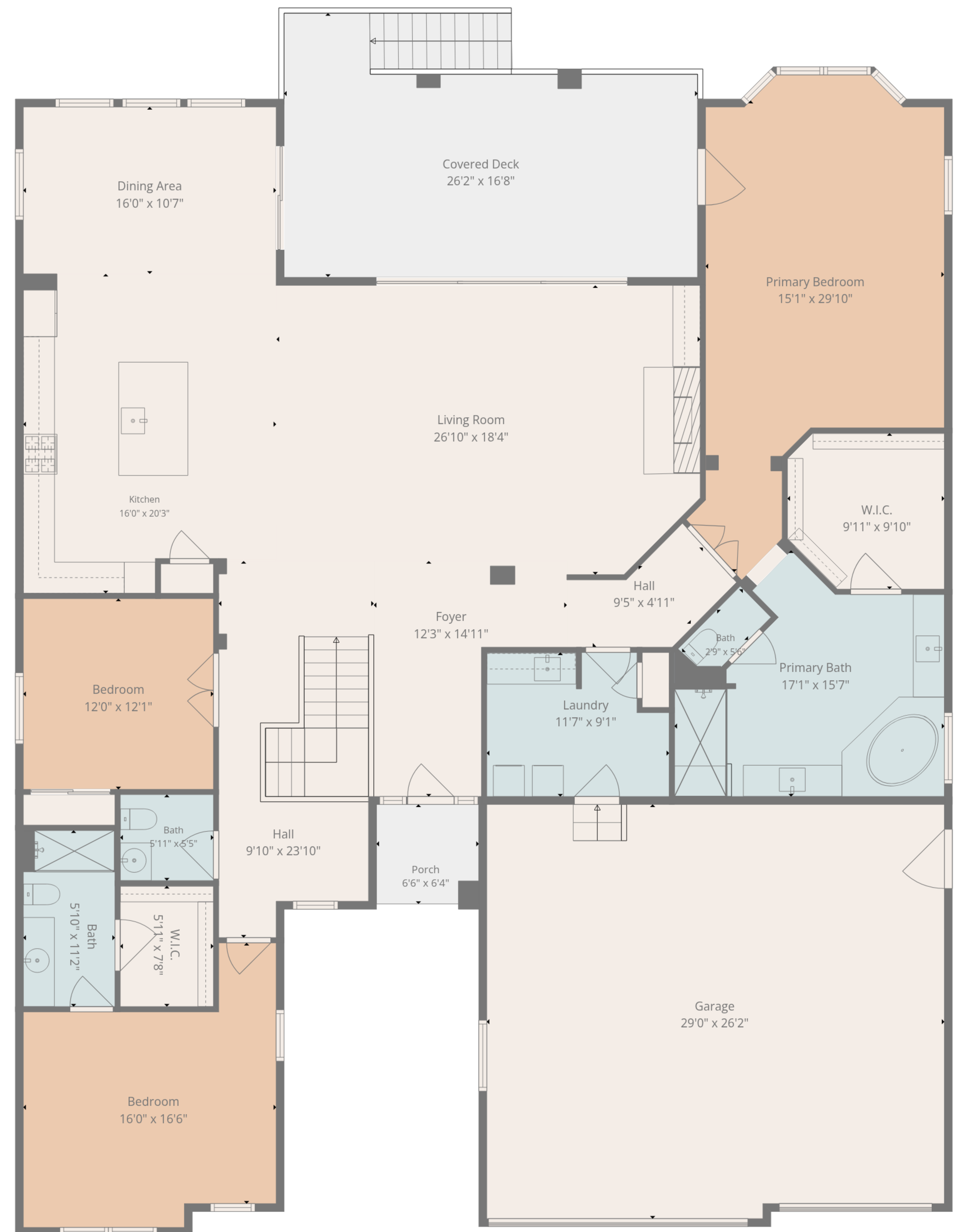
1st Floor
