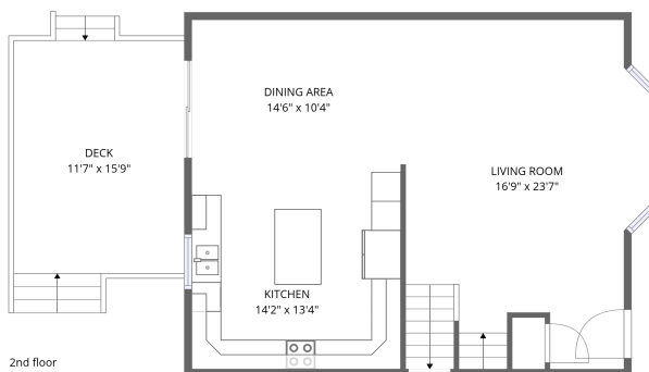
2nd floor
