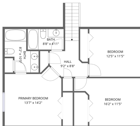
3rd floor
