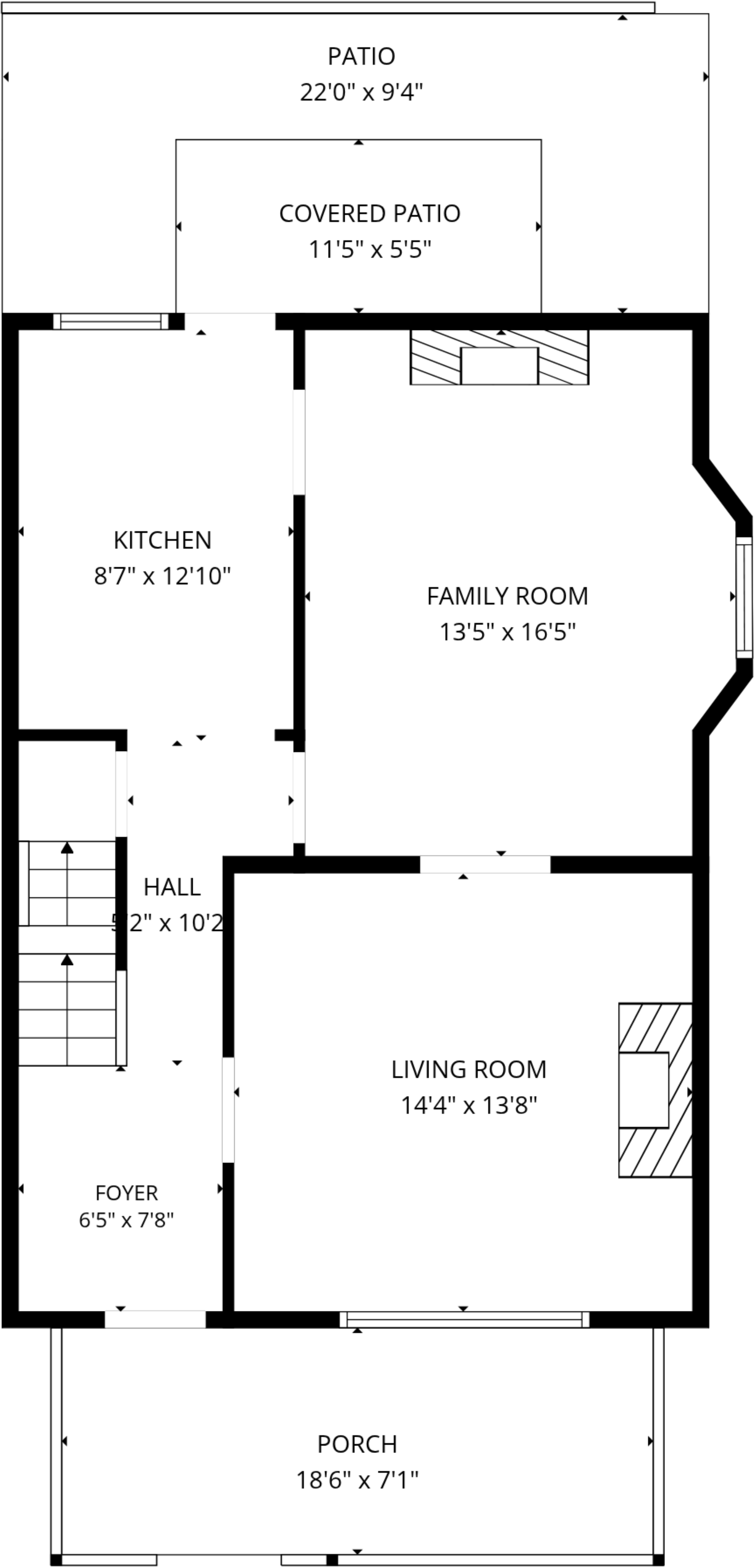
1st floor
