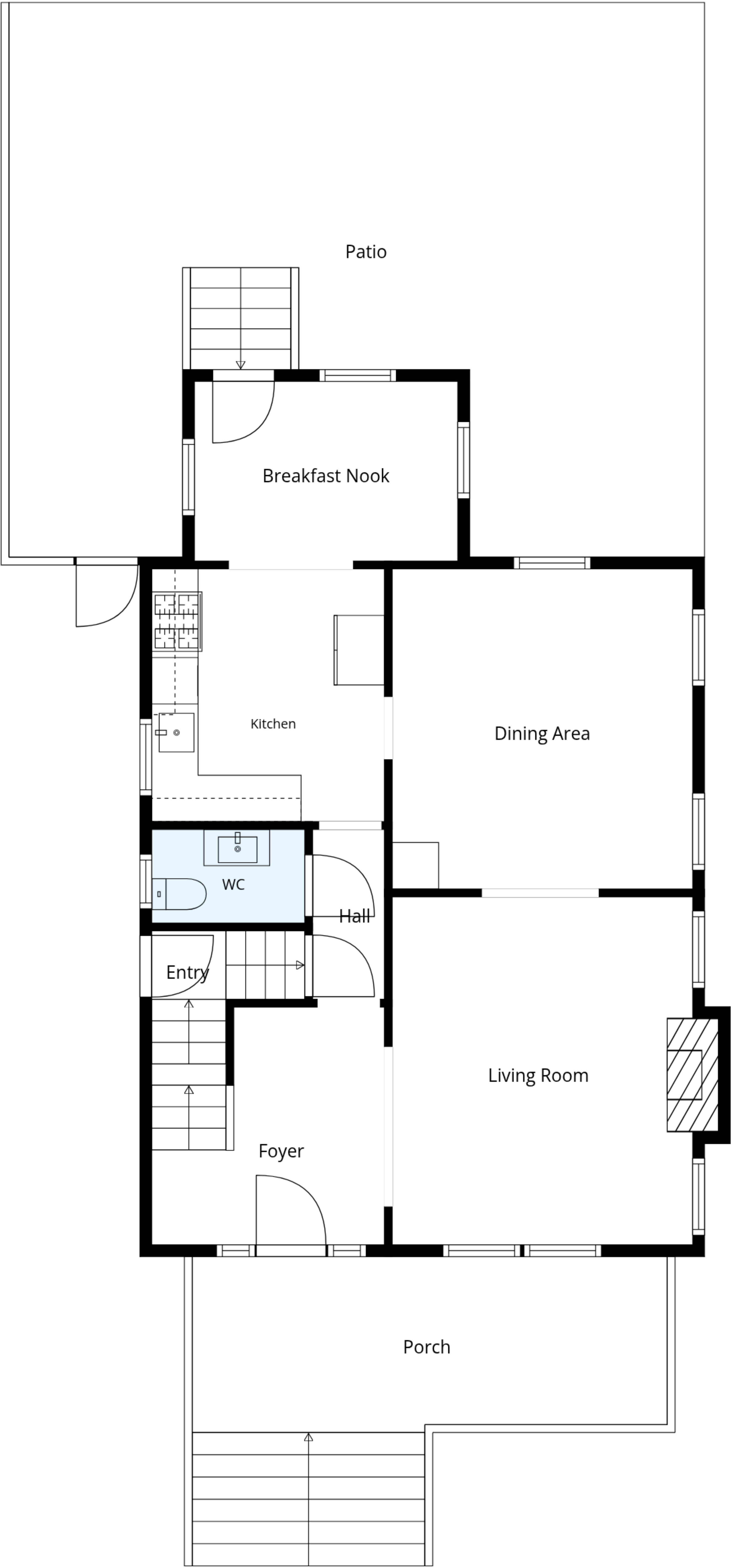
Ground Floor
