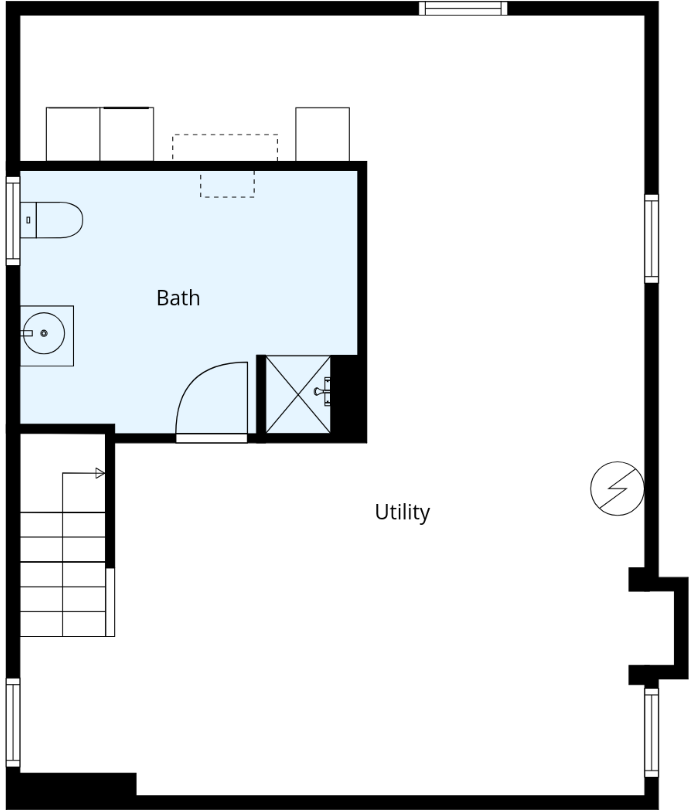
Basement
