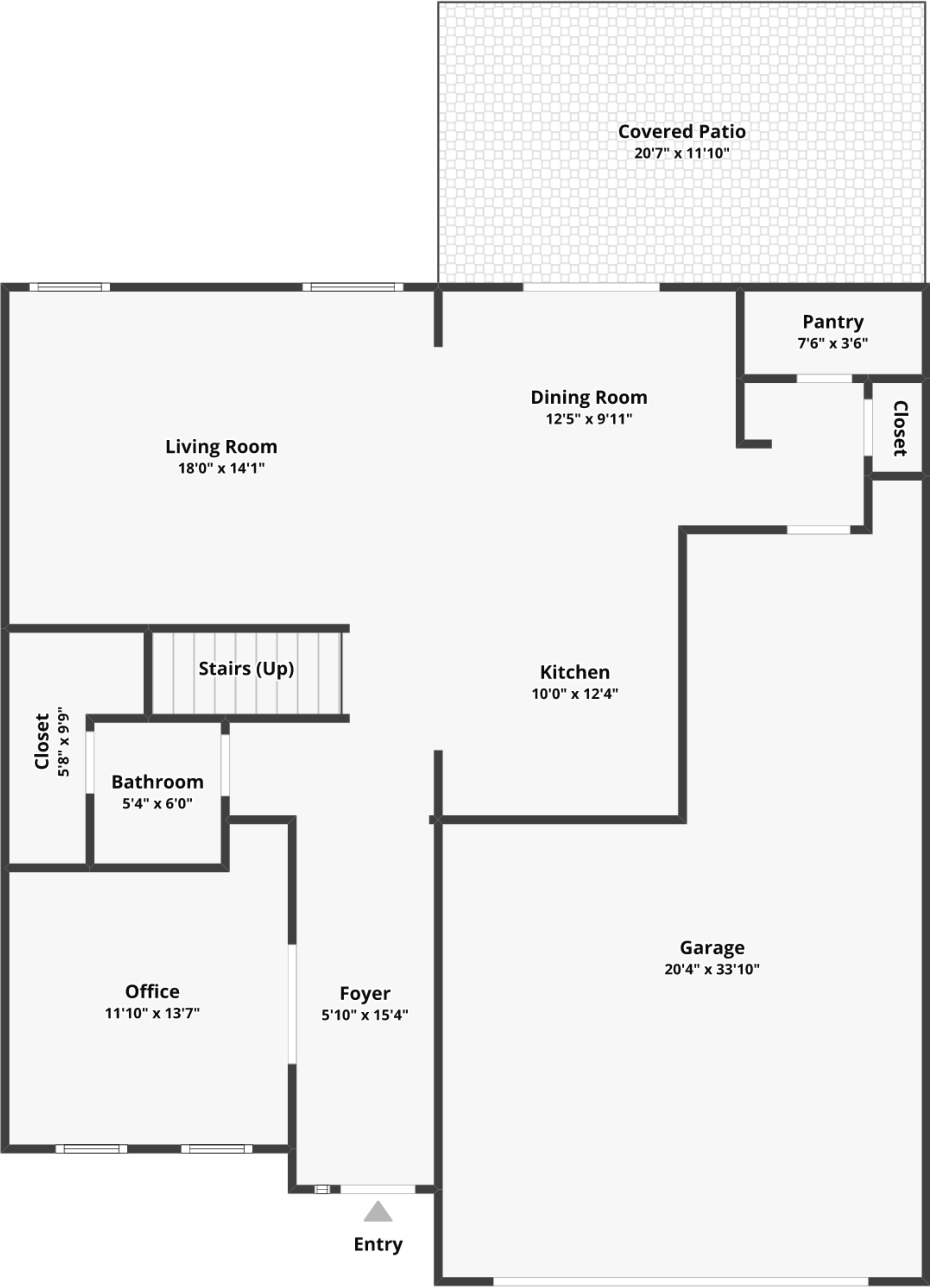
FLOOR 1
