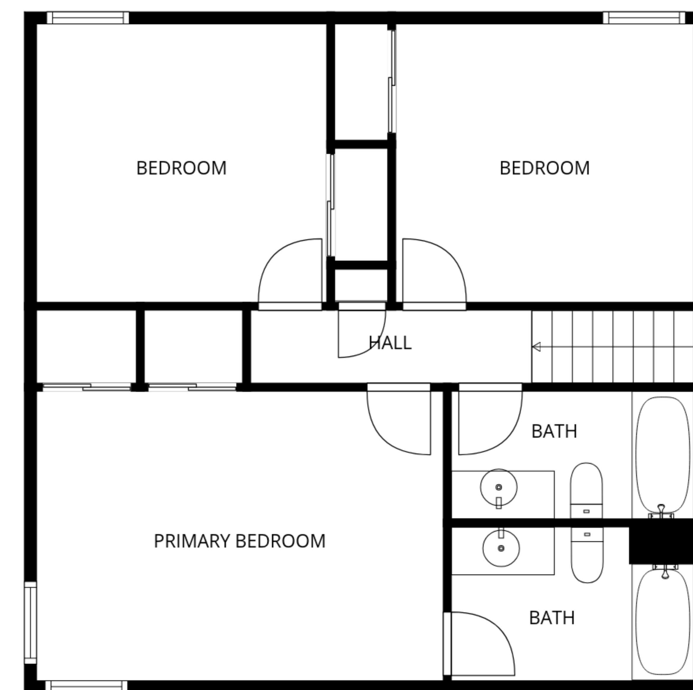
2nd floor
