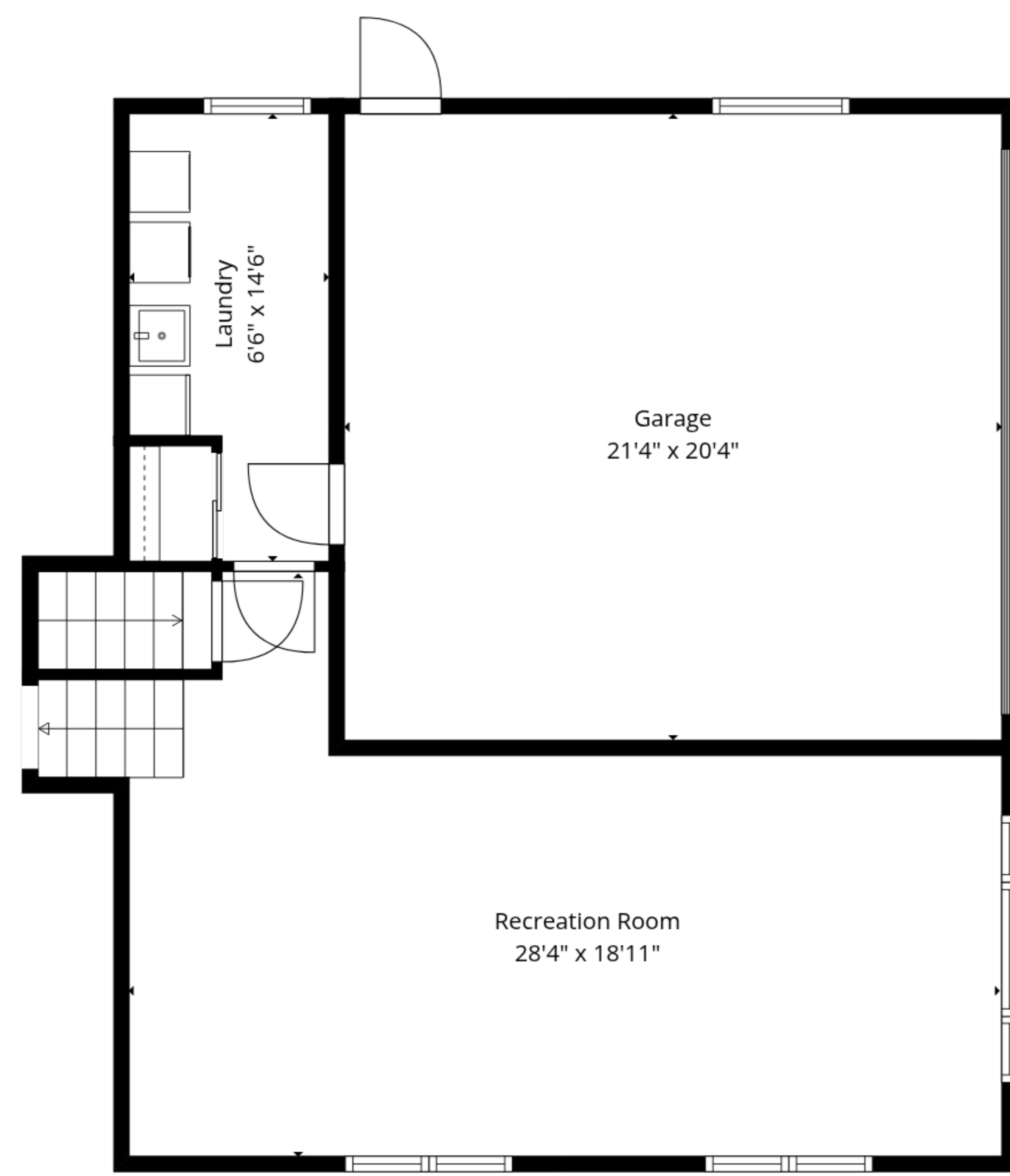
1st Floor
