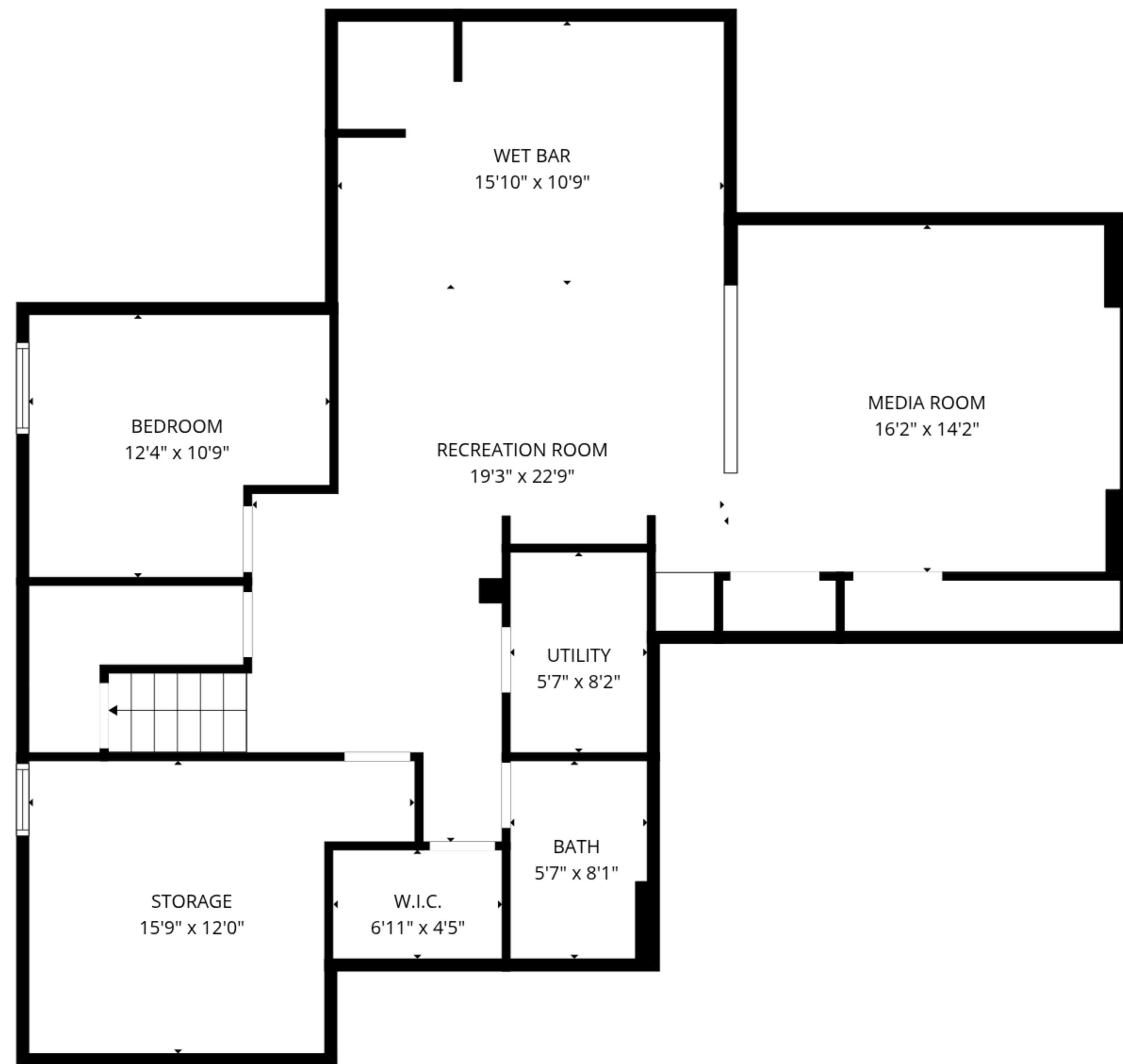
Basement 1
