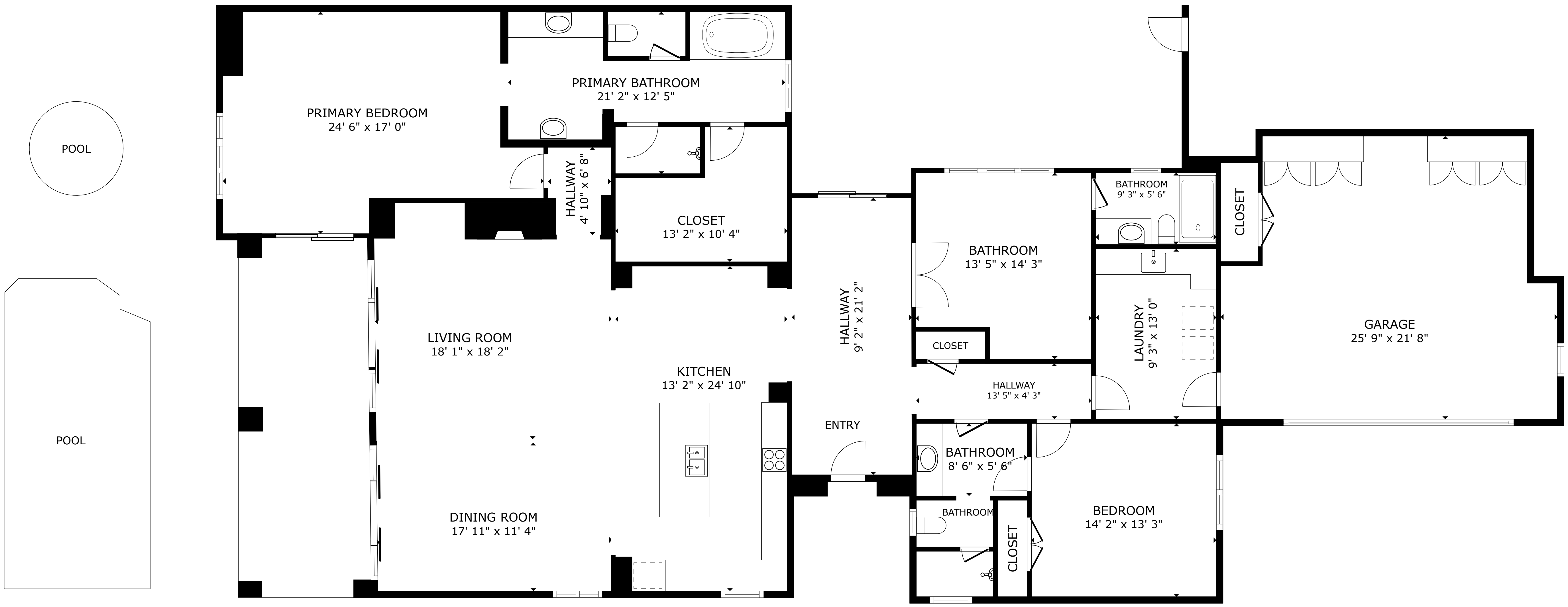
FLOOR PLAN
