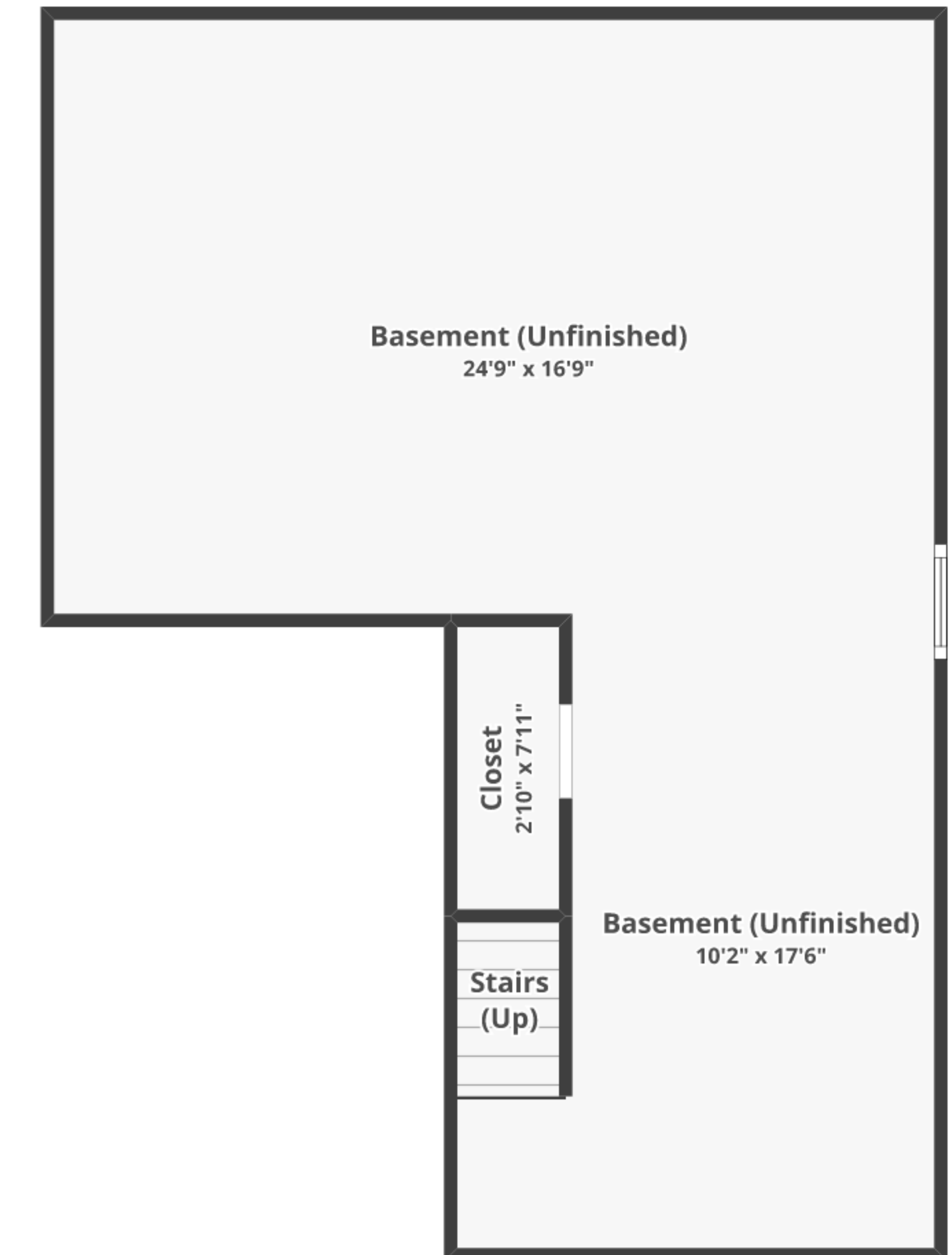
BASEMENT Finished area: ~22.75 sq. ft. Unfinished area: ~610.22 sq. ft.
