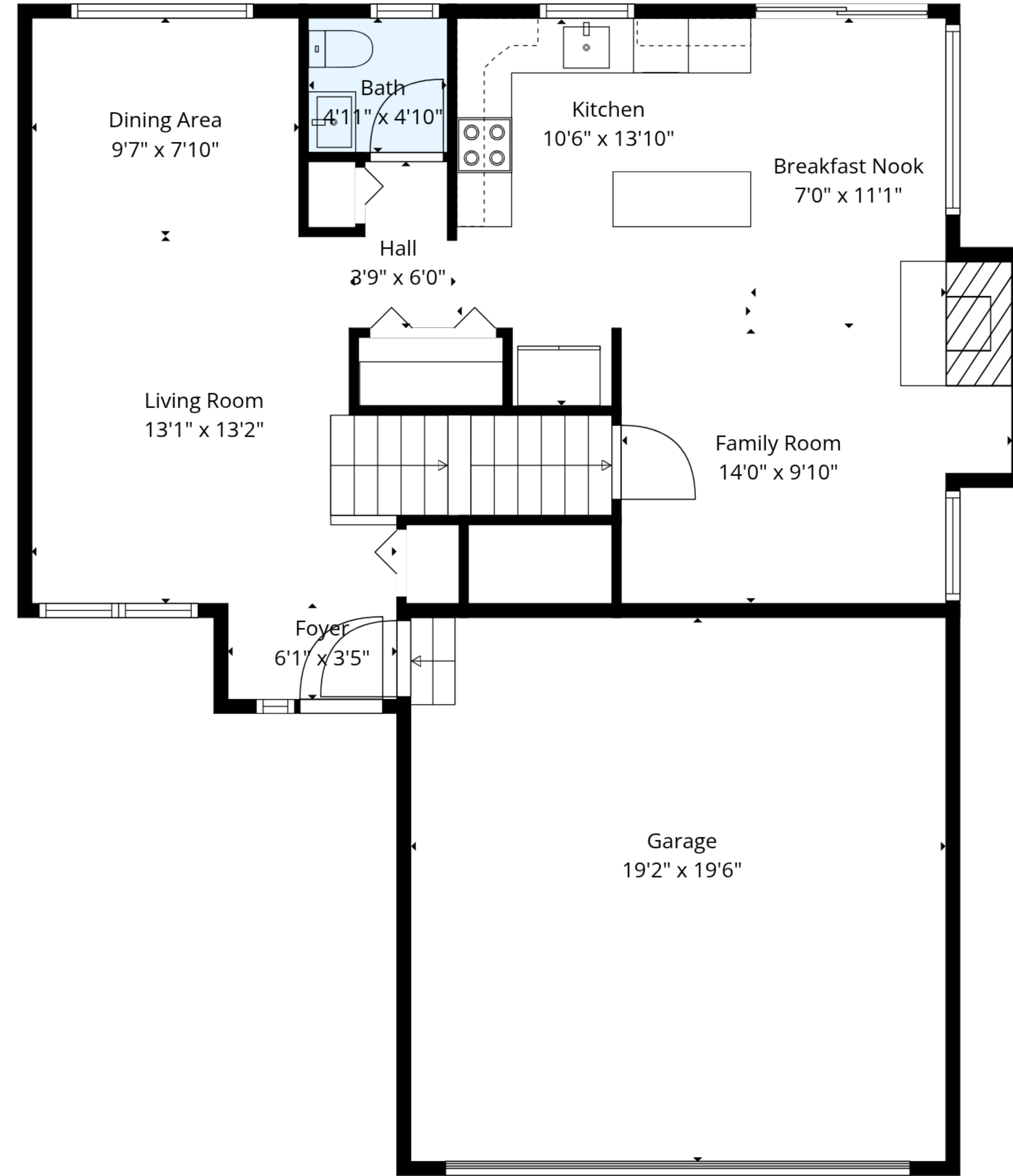
1st Floor
