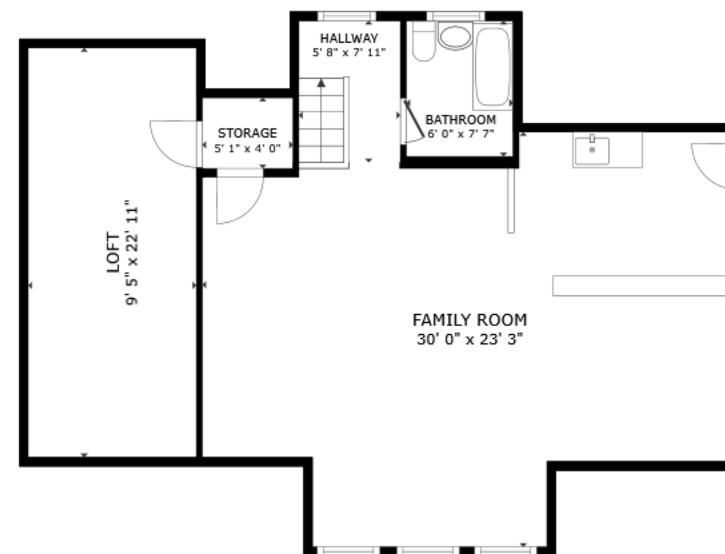
FLOOR 2
