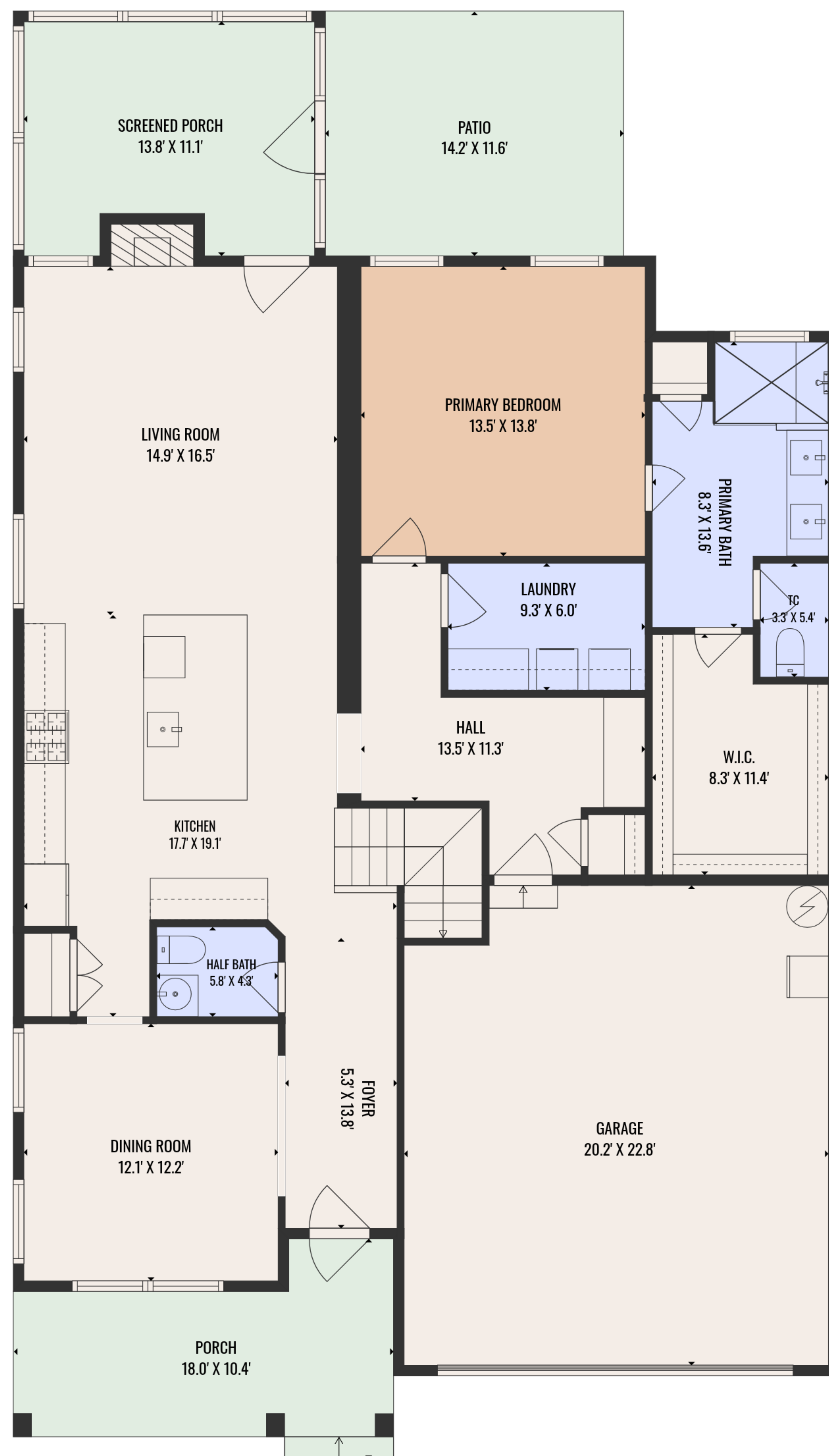
1ST FLOOR
