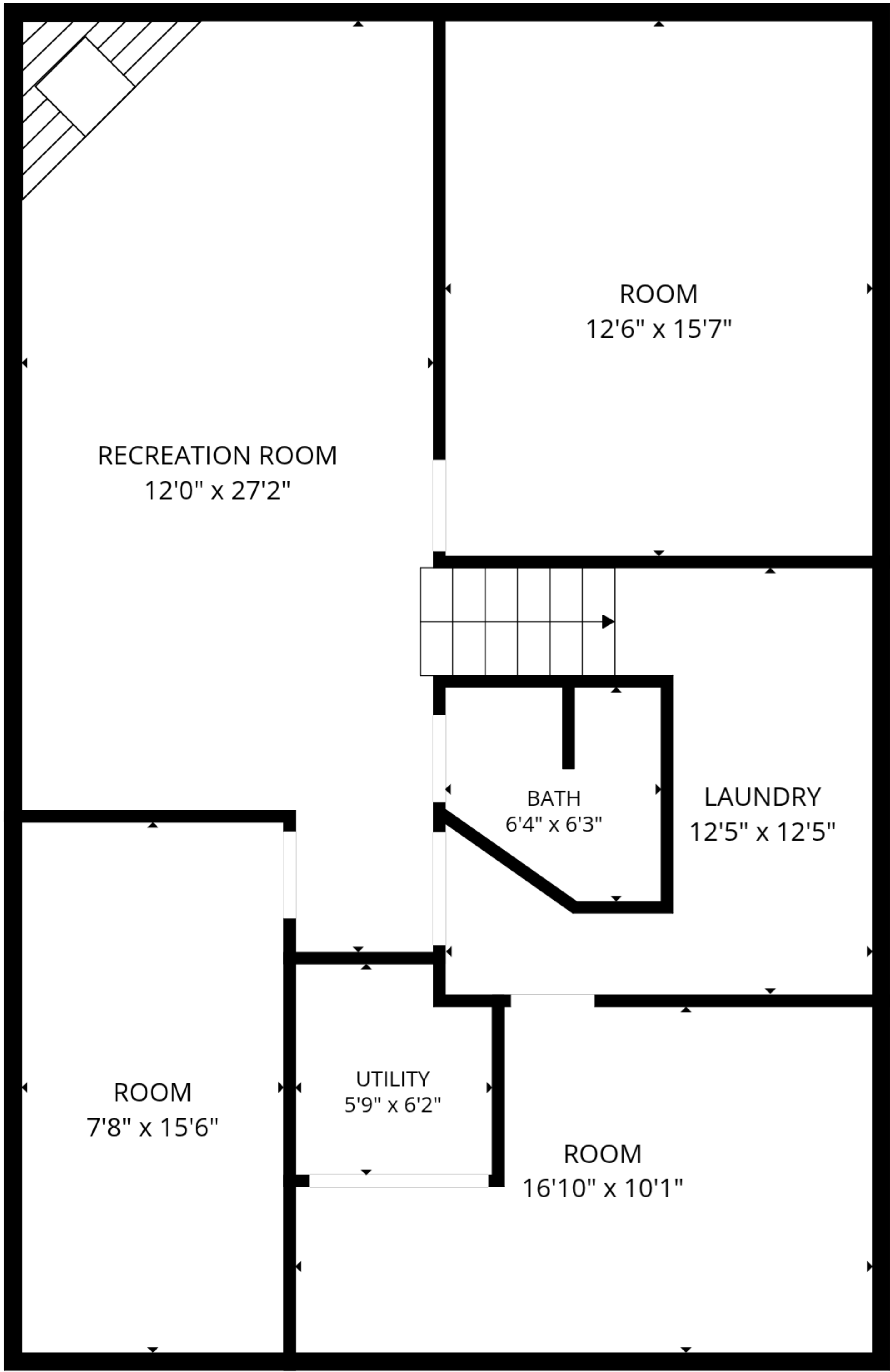
Basement
