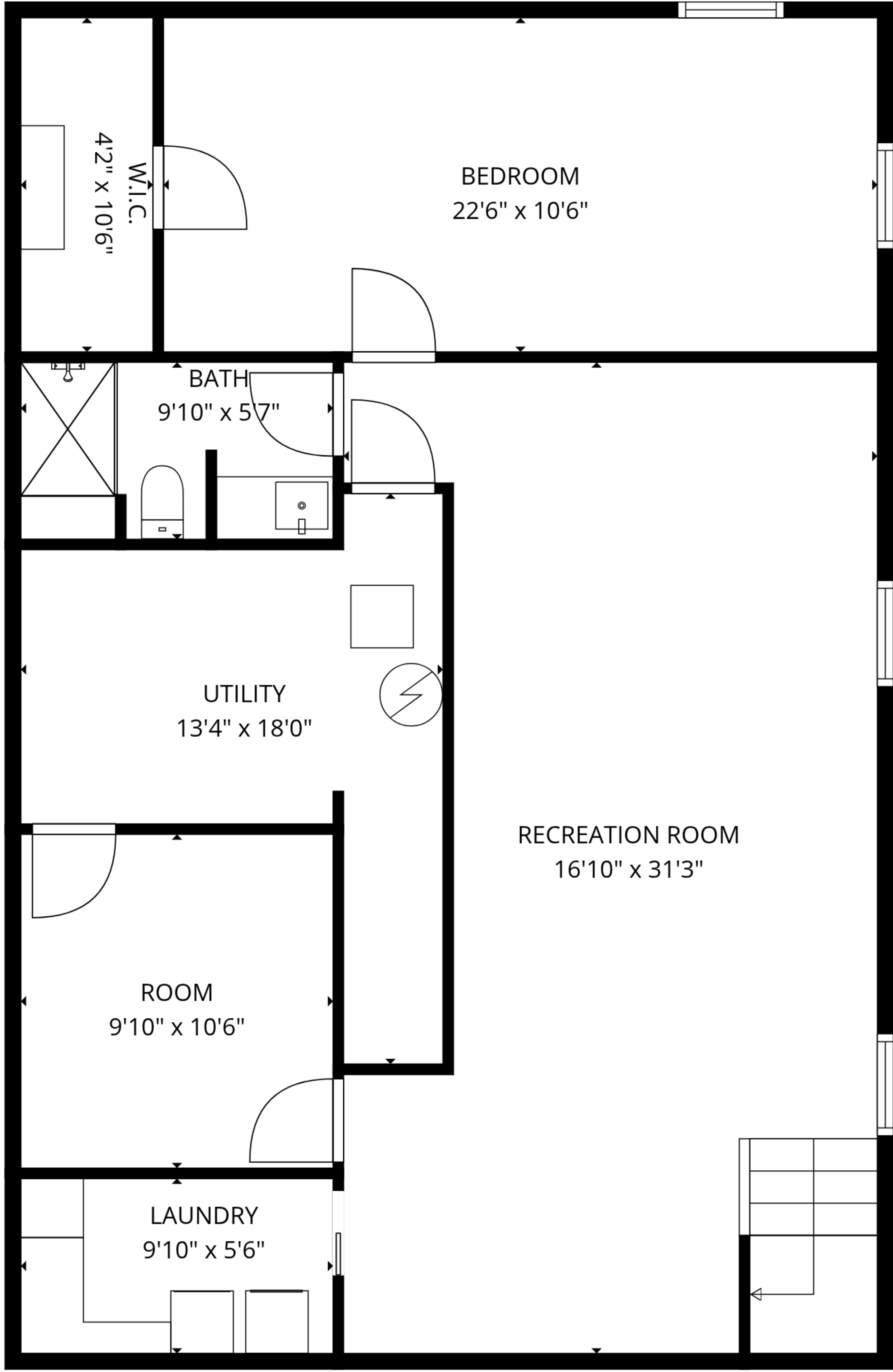
Basement 1
