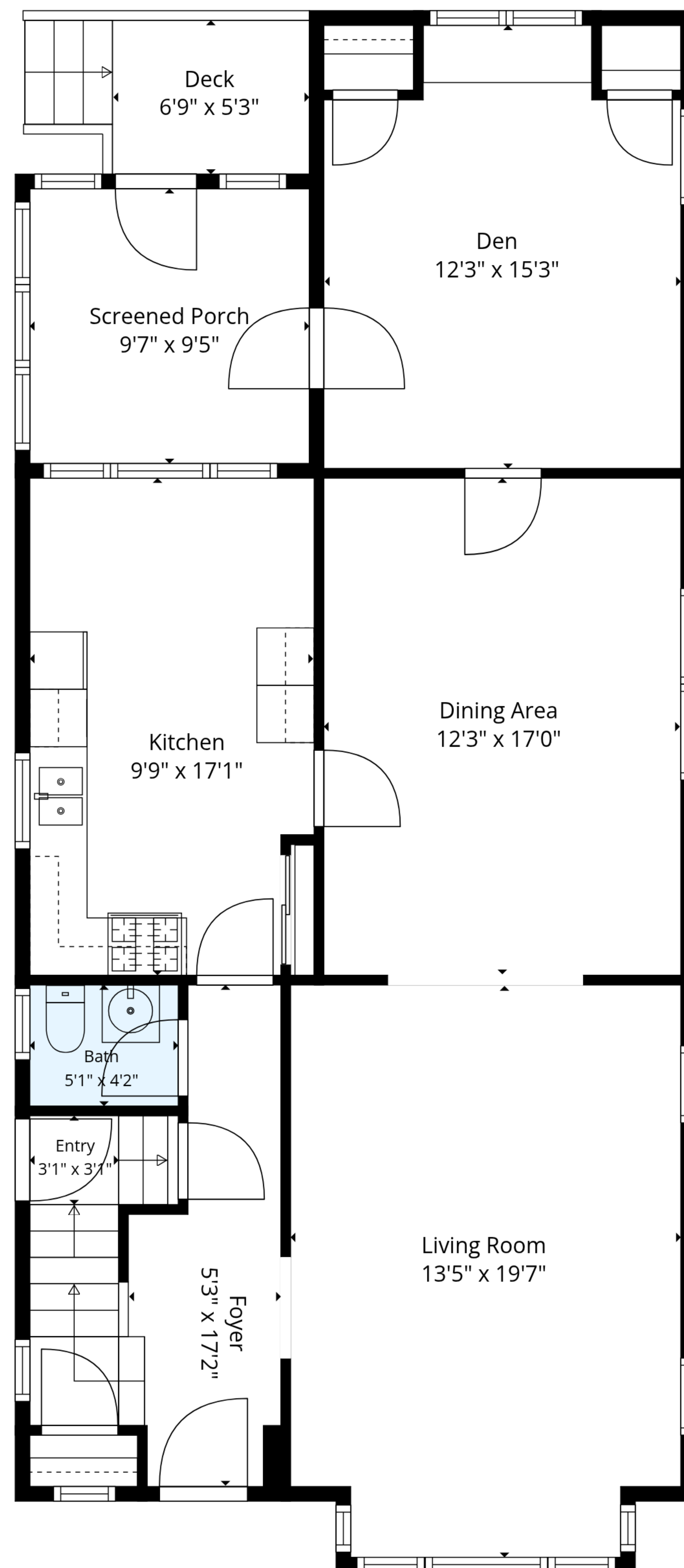
1st Floor
