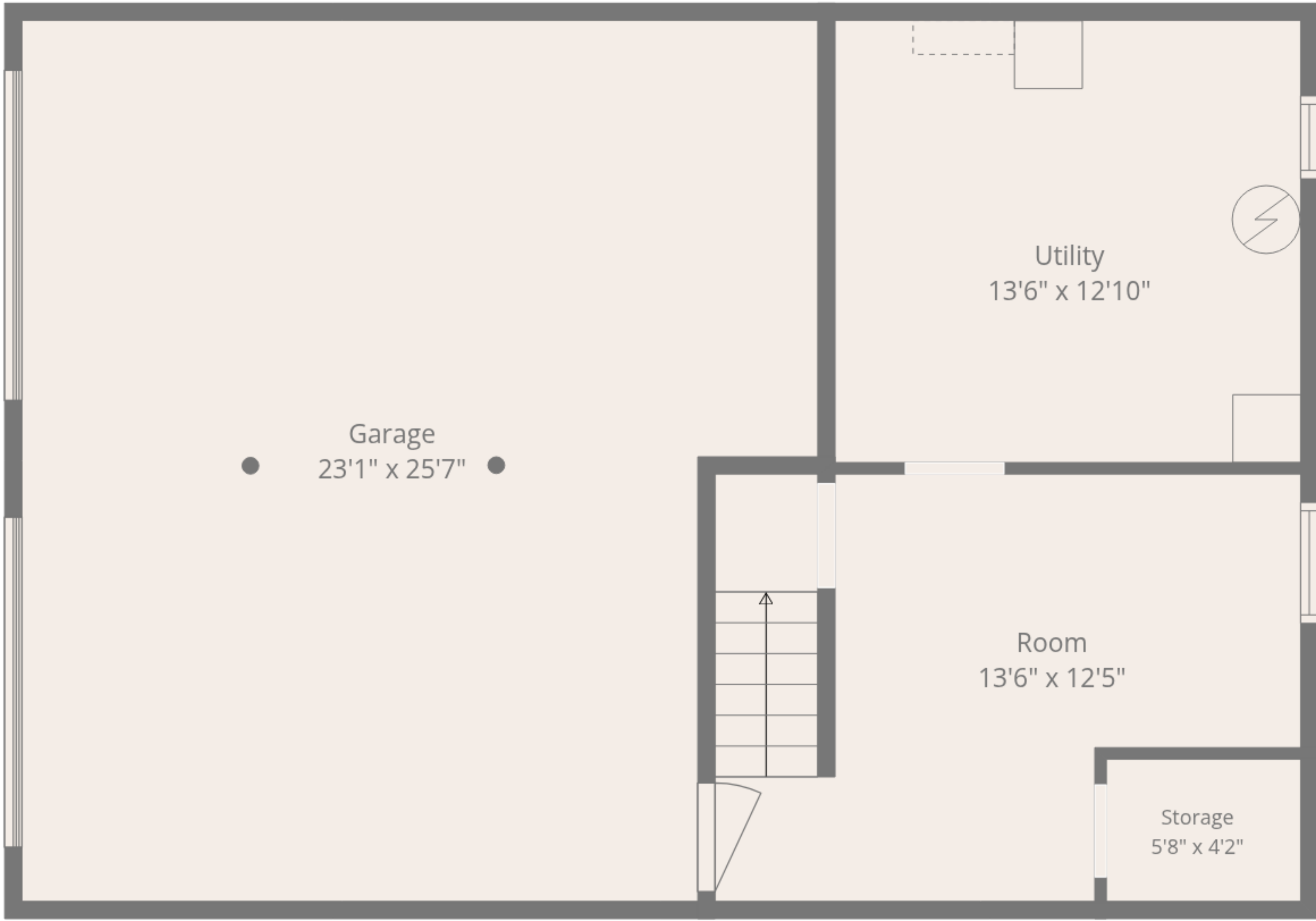
Basement
