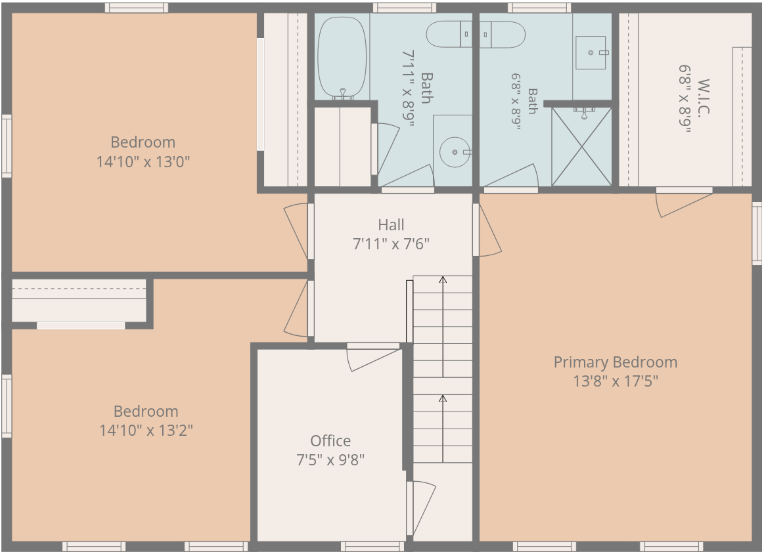
2nd Floor
