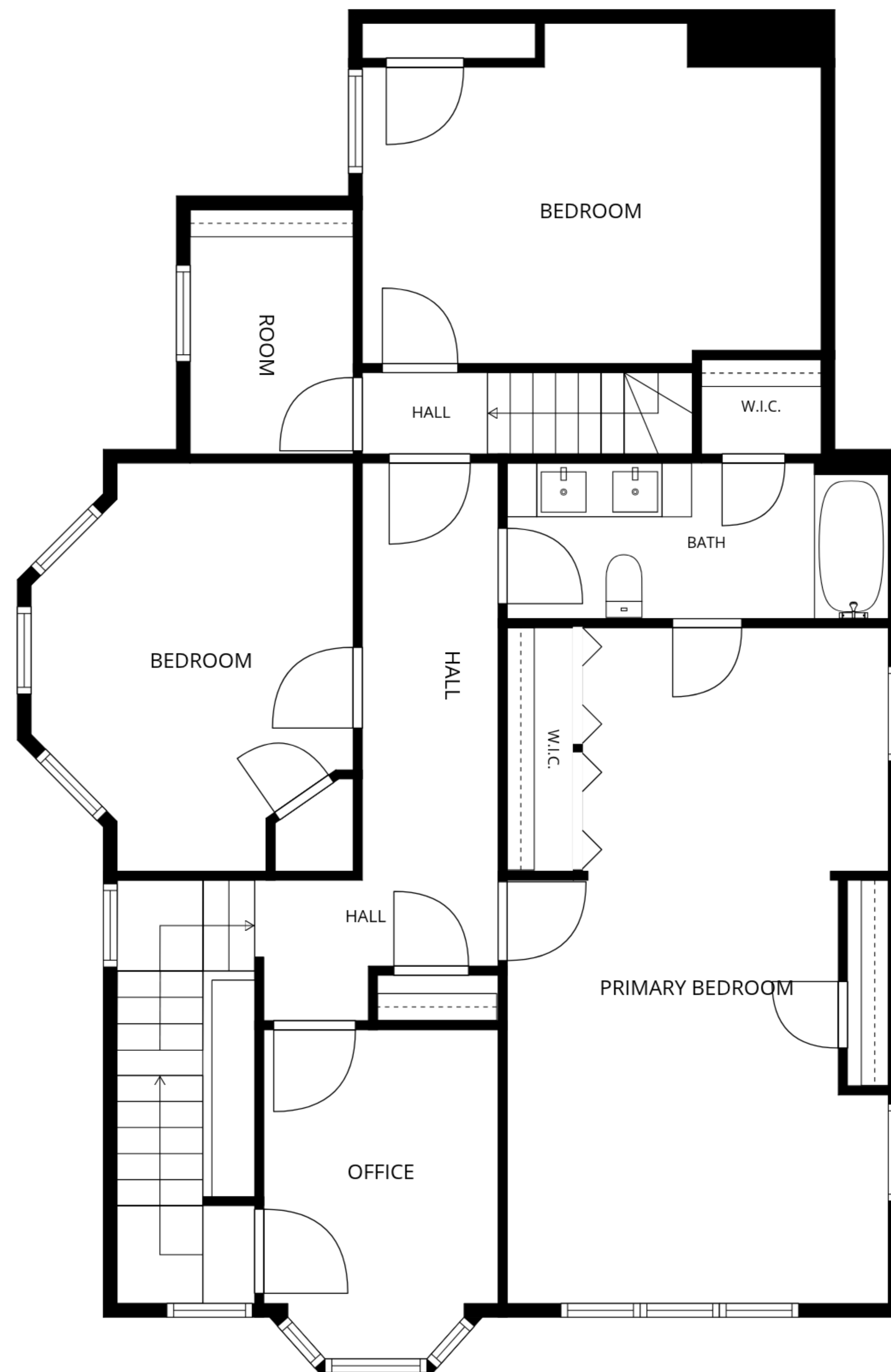
2nd floor
