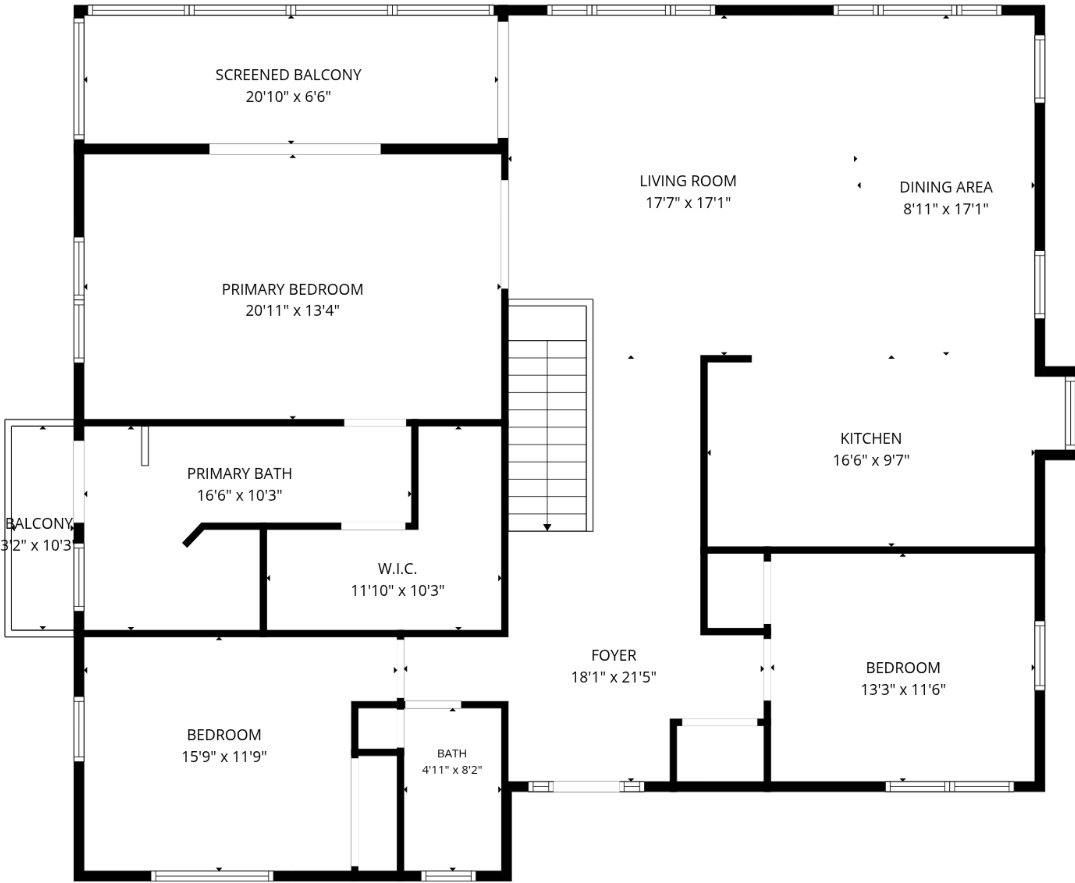
2nd floor
