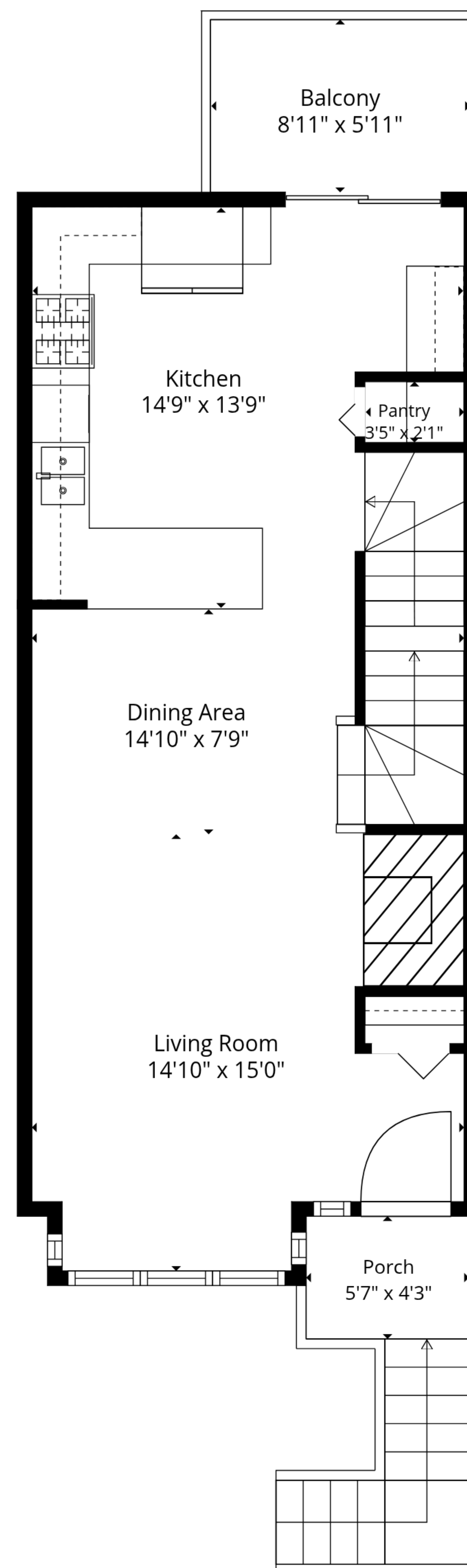
1st Floor
