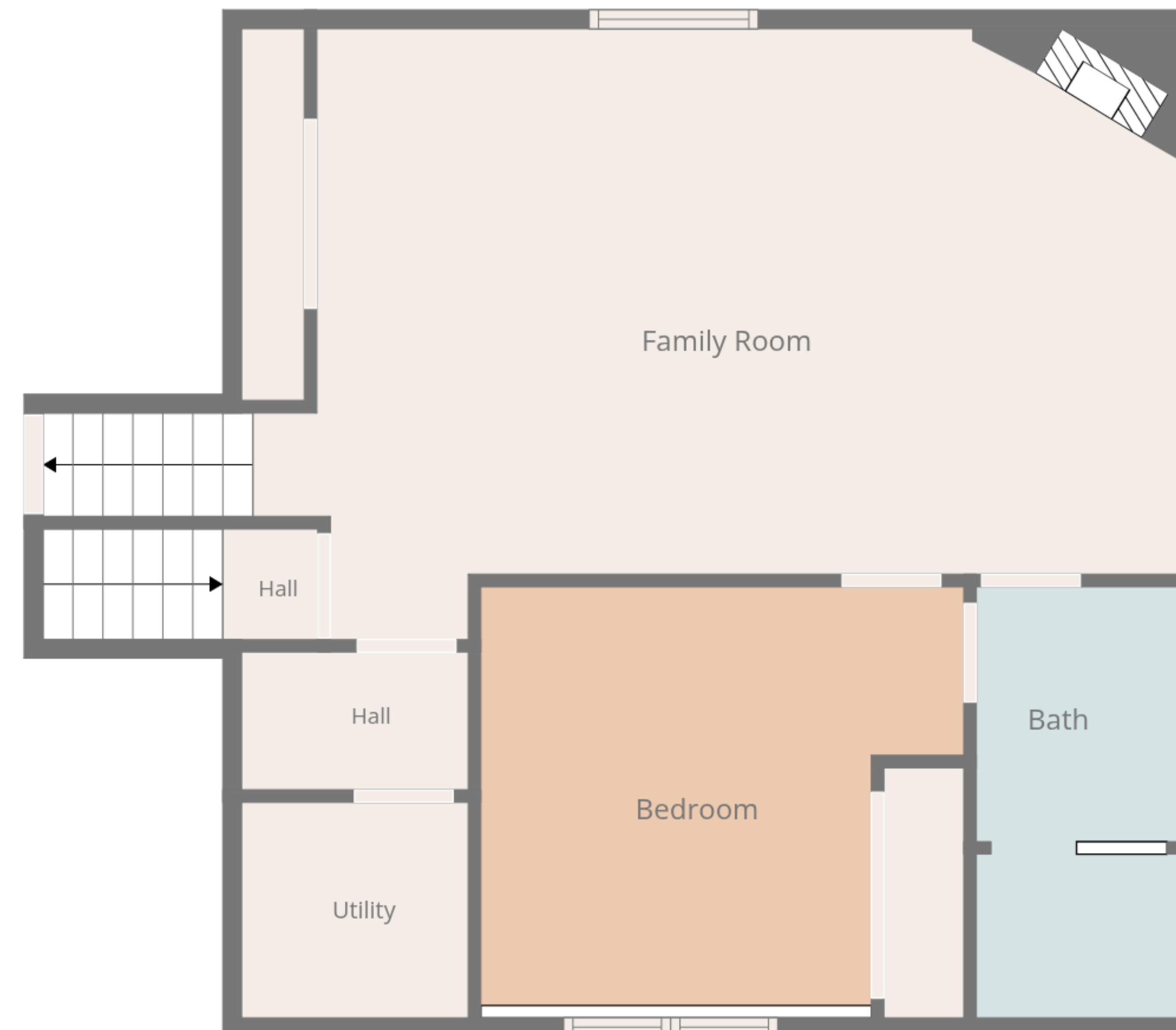
2nd Floor
