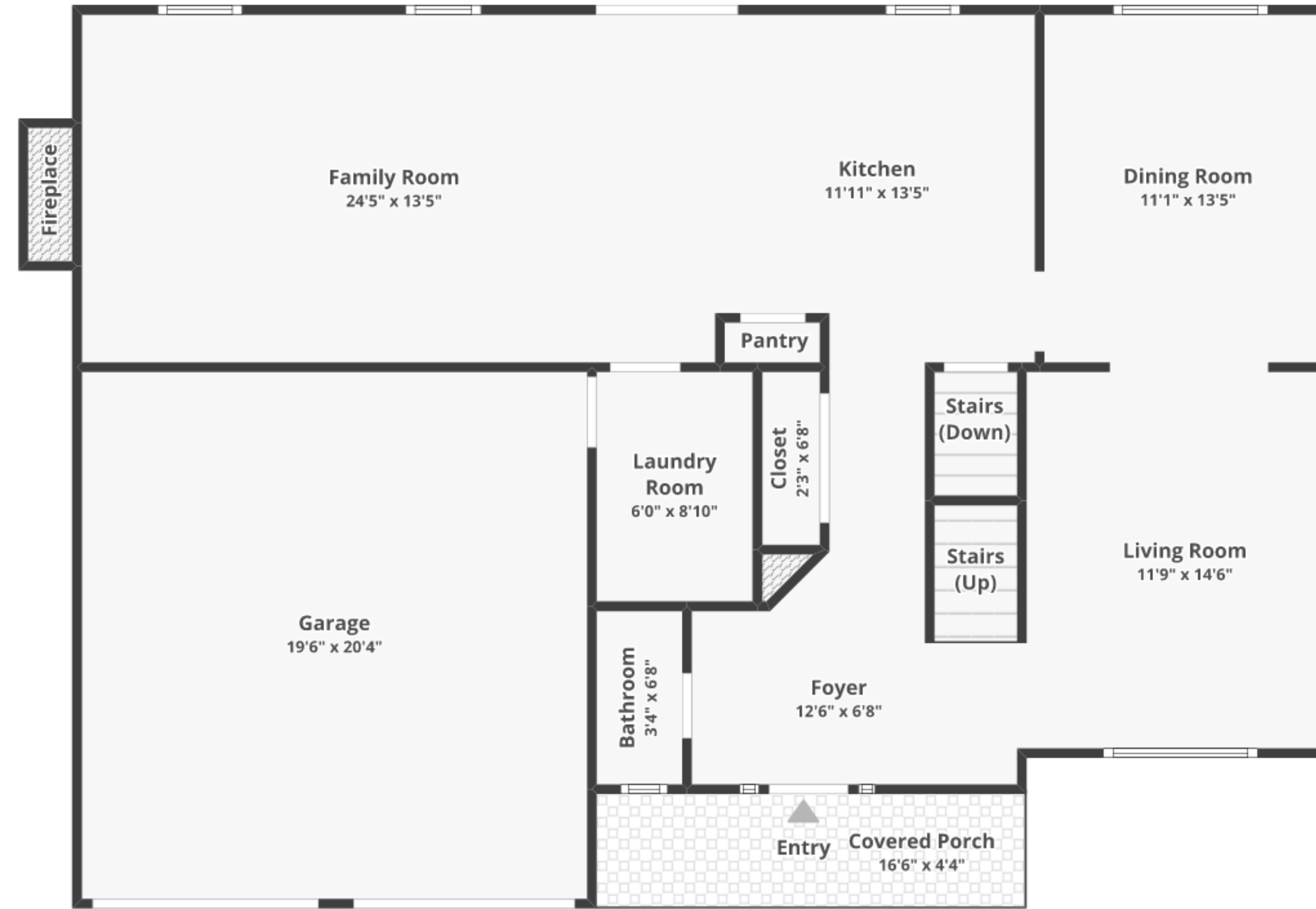
FLOOR 1 Finished area: ~1,047.57 sq. ft. Unfinished area: ~10.59 sq. ft.
