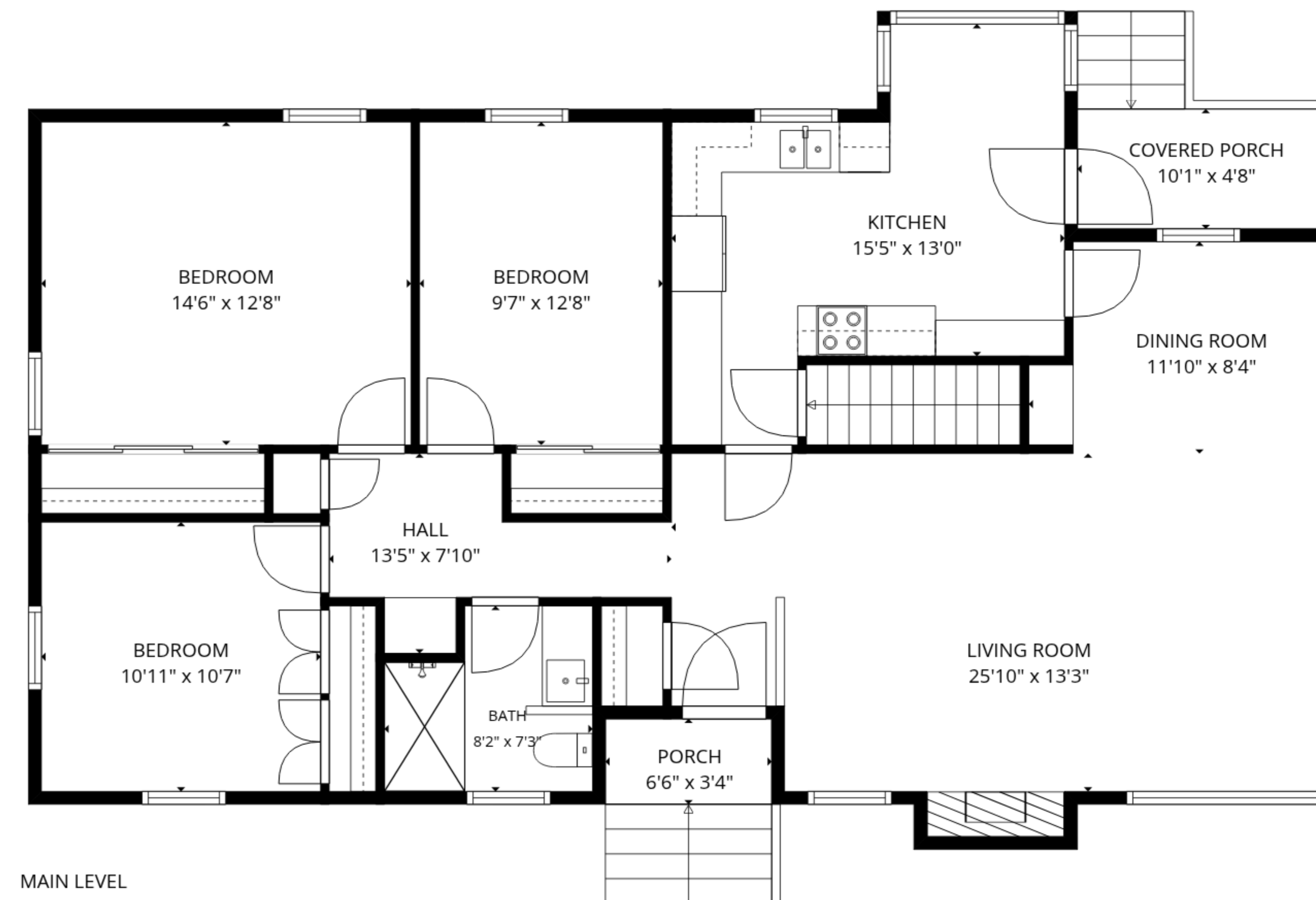
MAIN LEVEL
