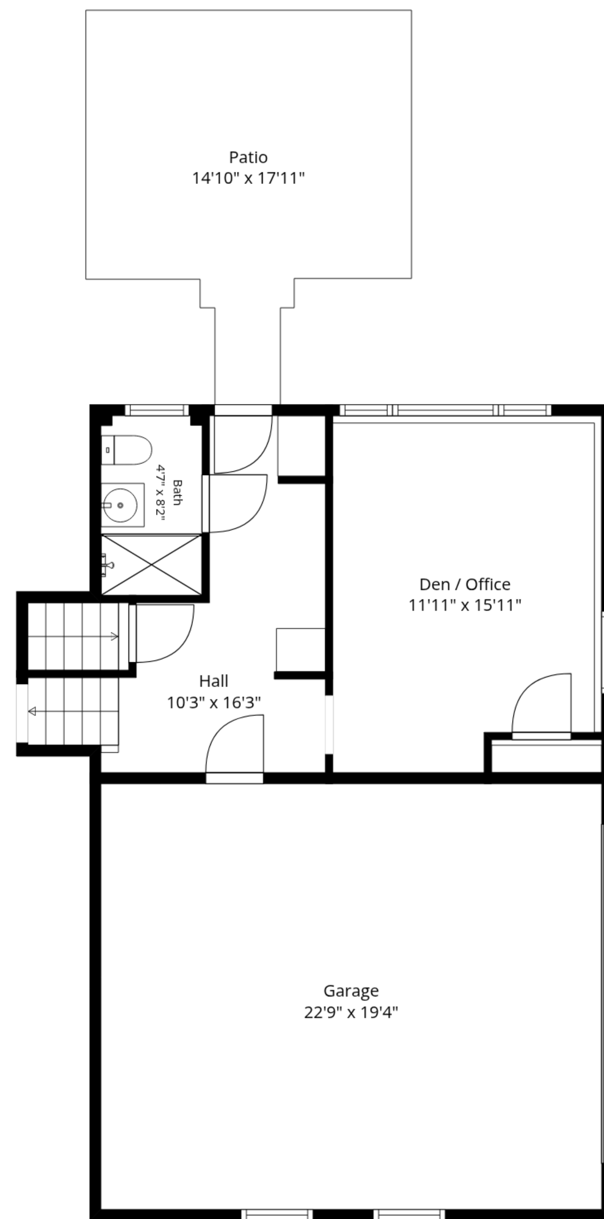
1st Floor
