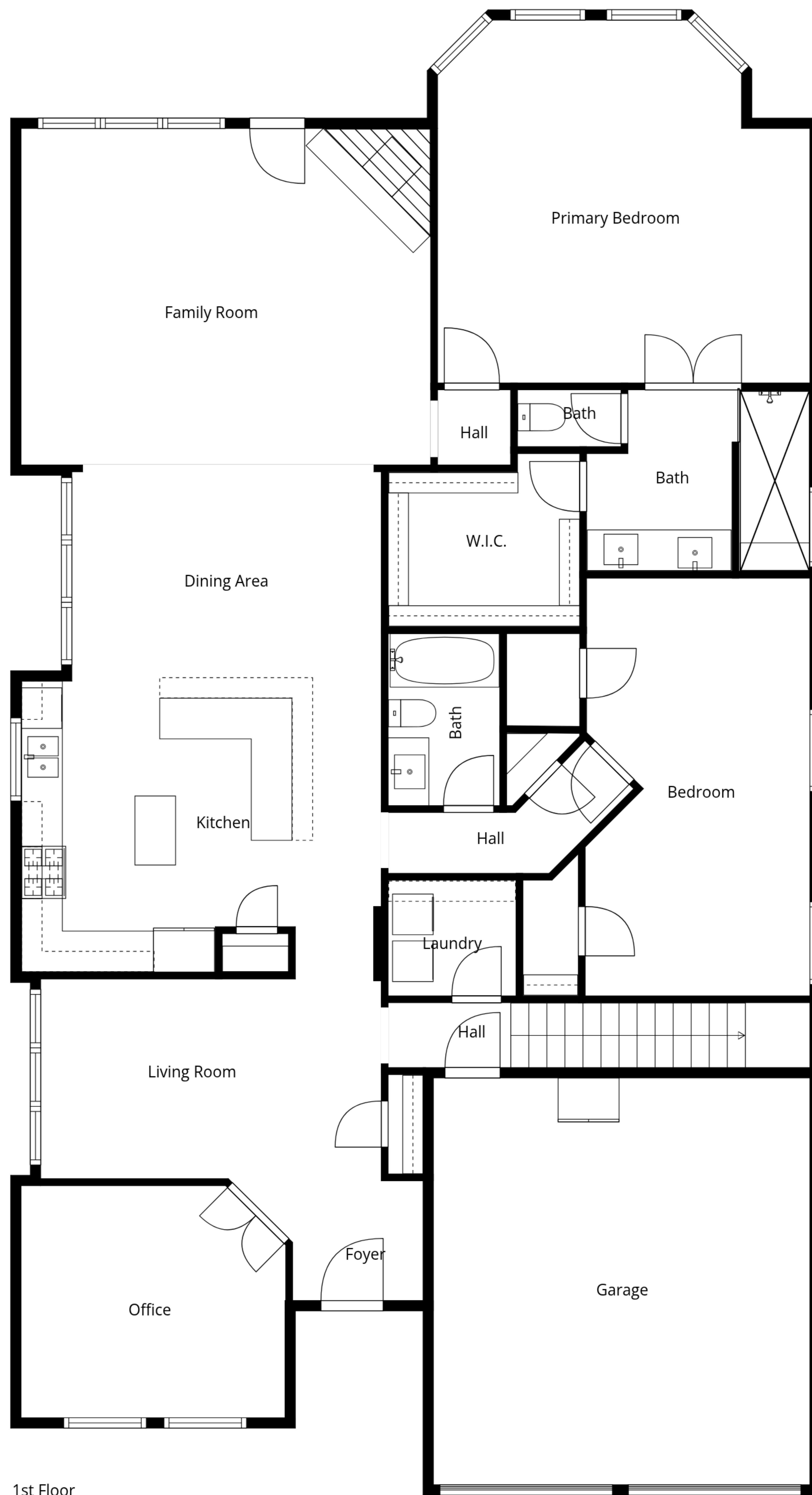
1st Floor
