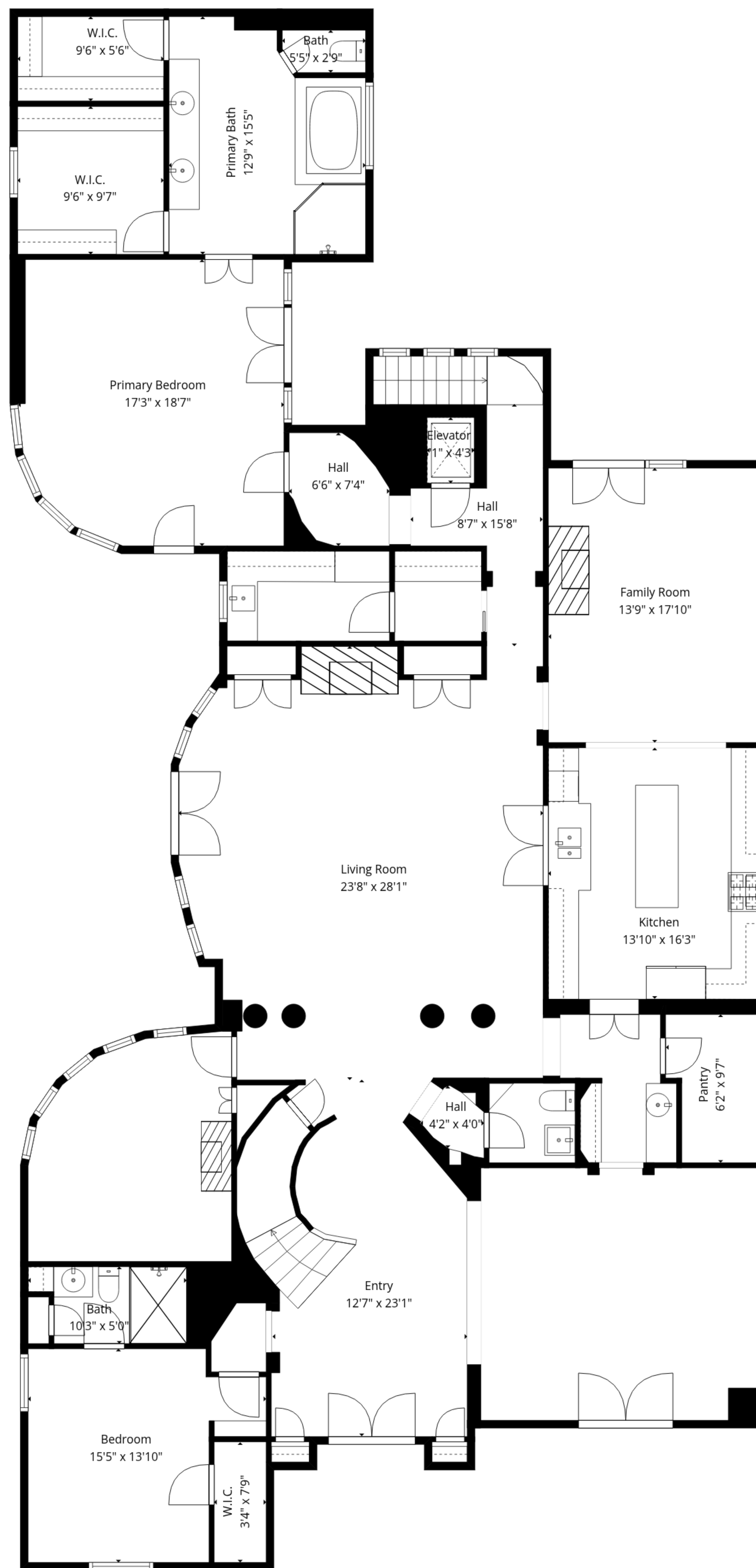
Floor 2
