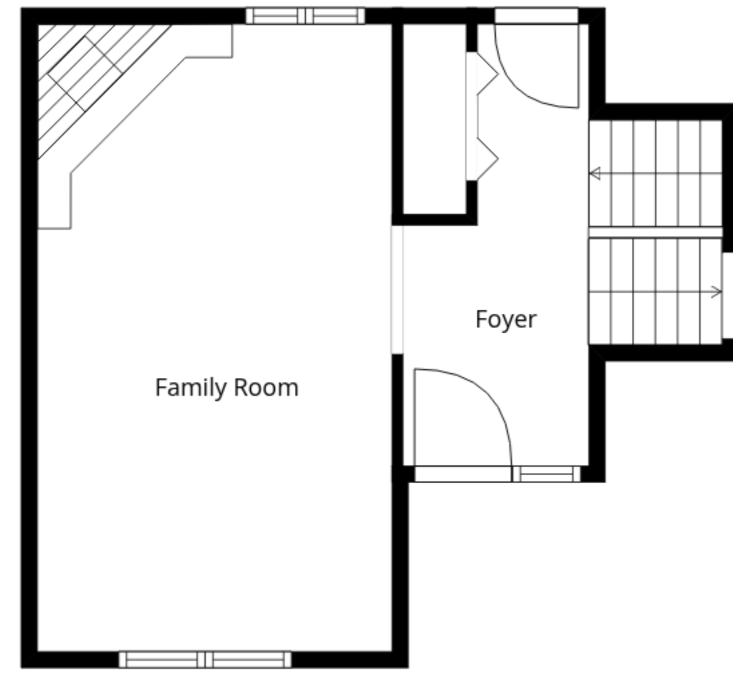
1st Floor
