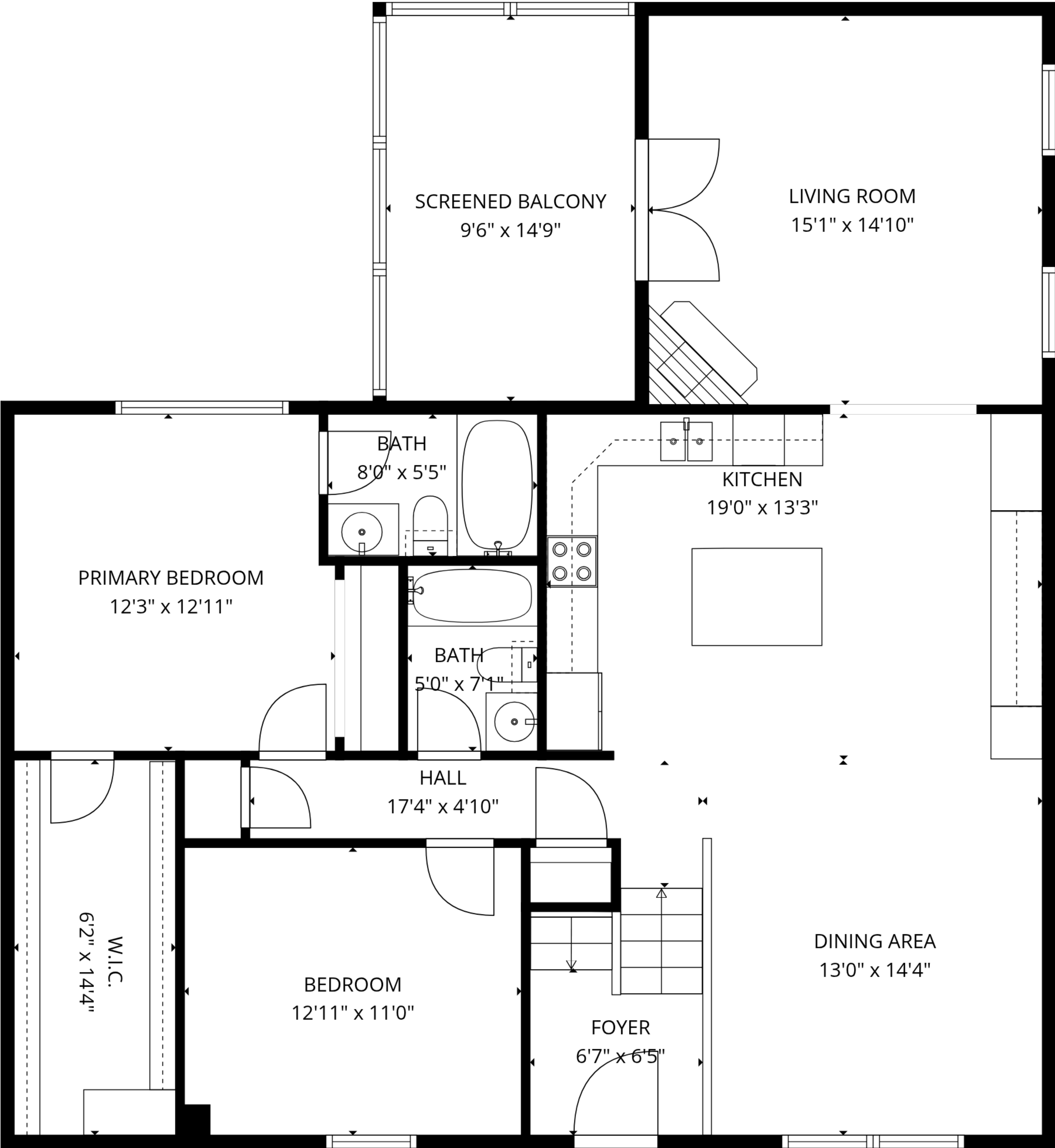
1st floor
