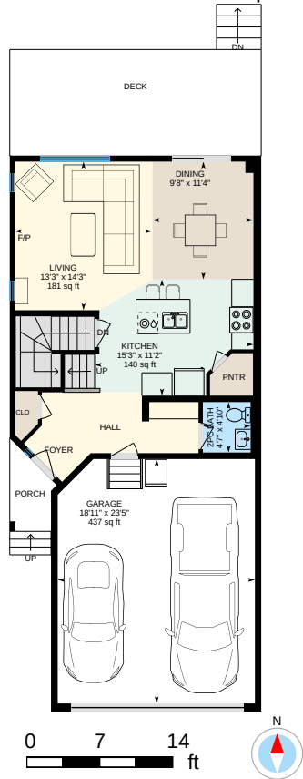
Main Floor Exterior Area 701.09 sq ft
