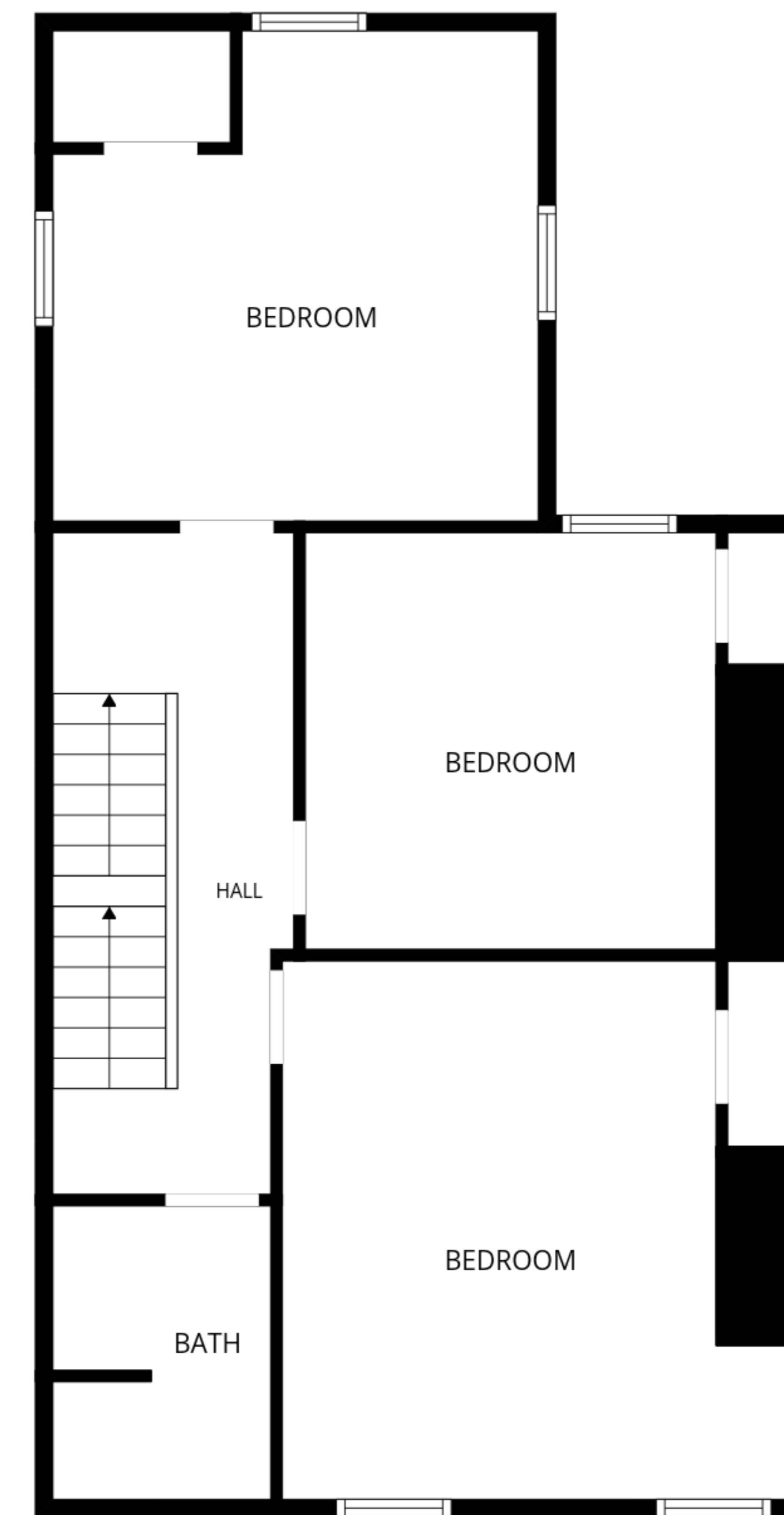
2nd floor
