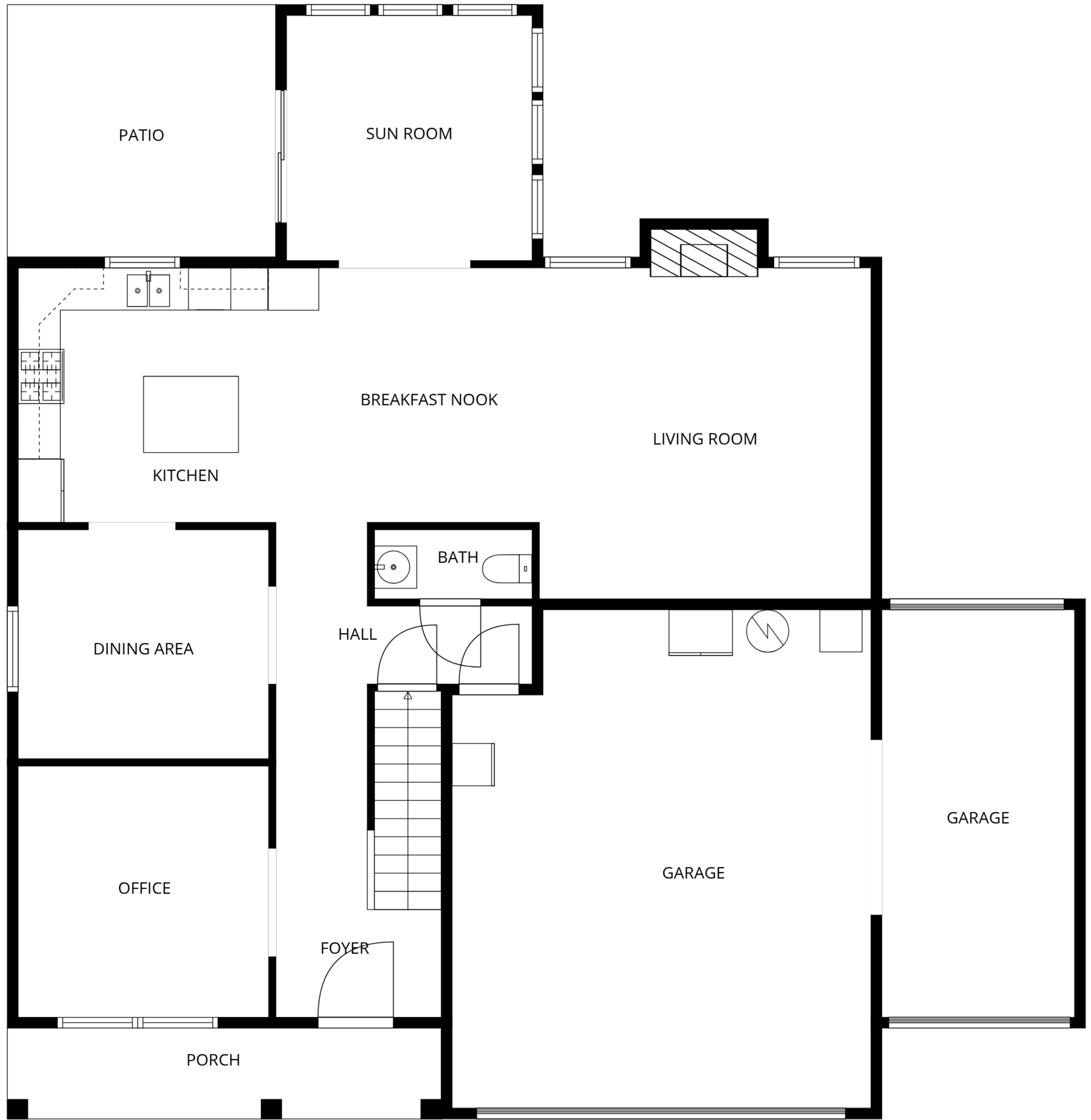
1st floor
