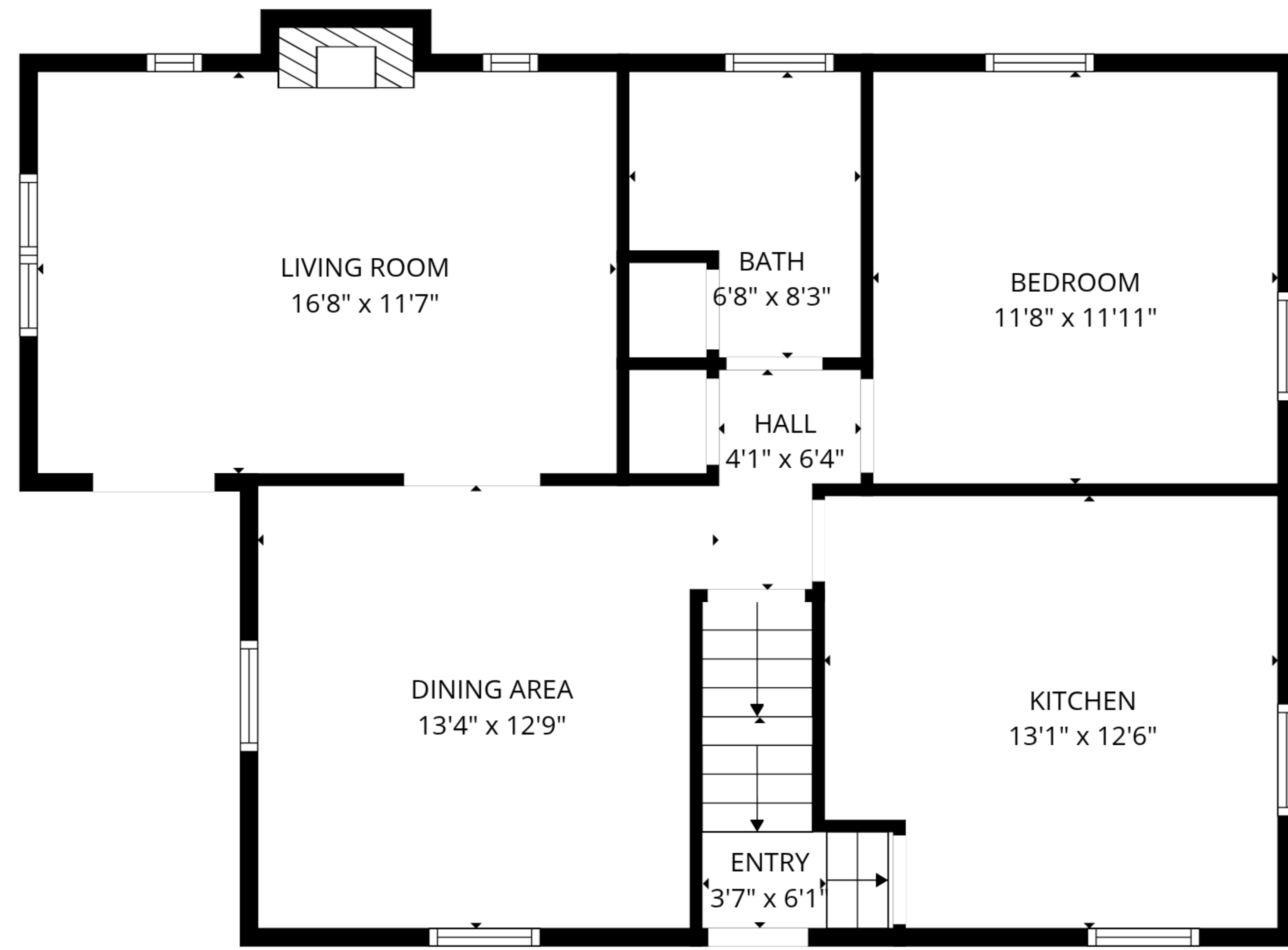
1st floor
