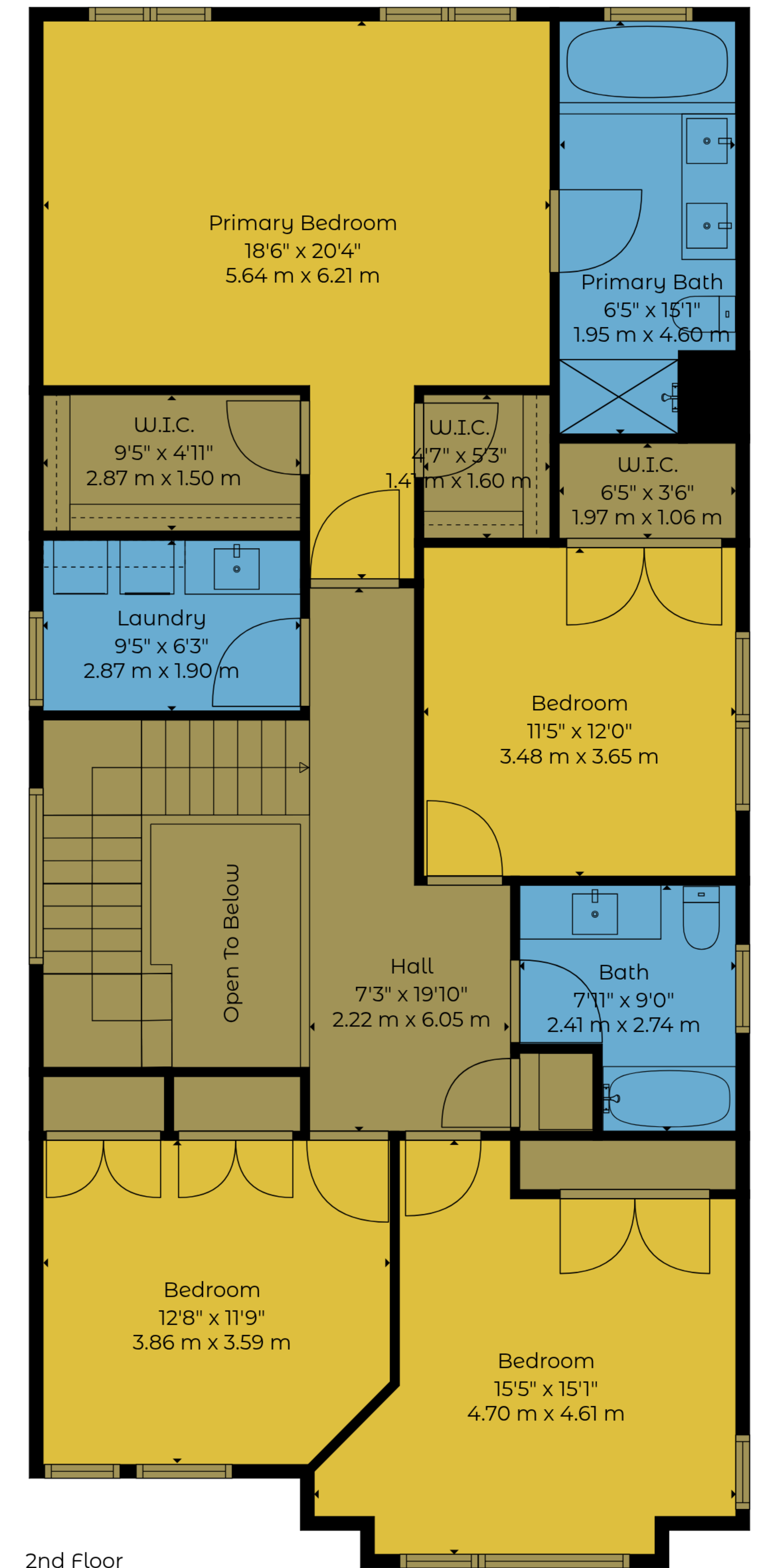
2nd Floor
