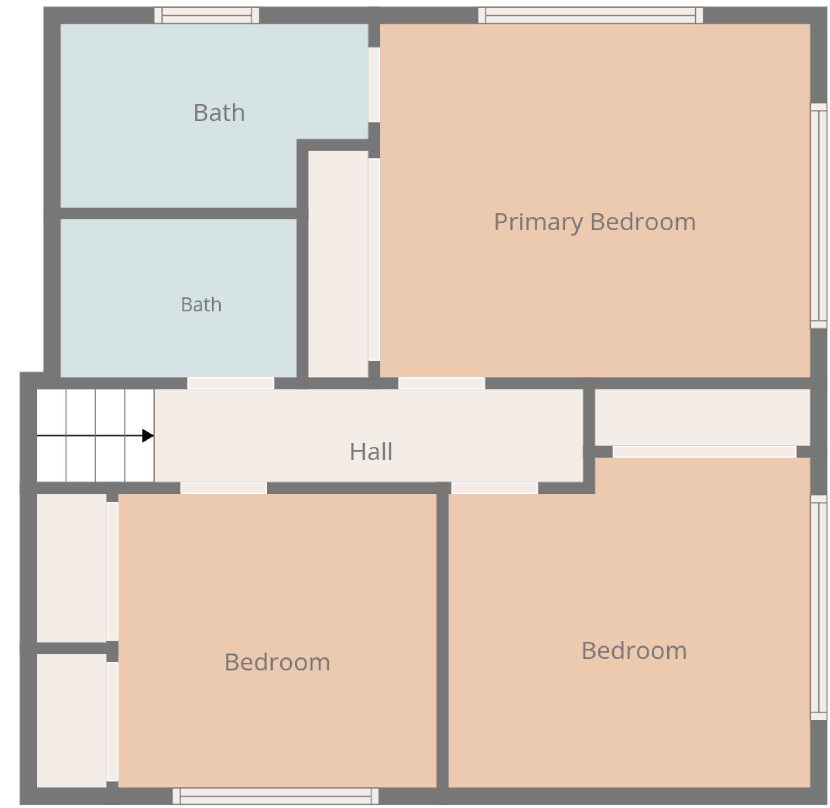
2nd Floor
