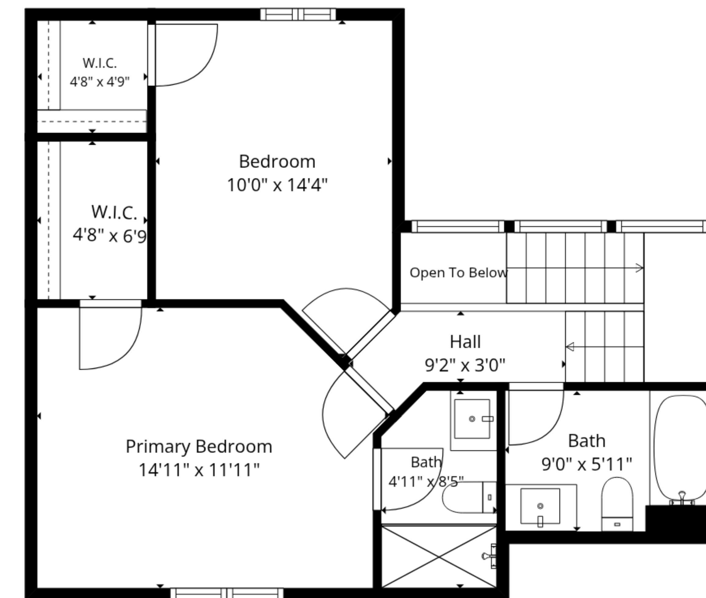
2nd Floor
