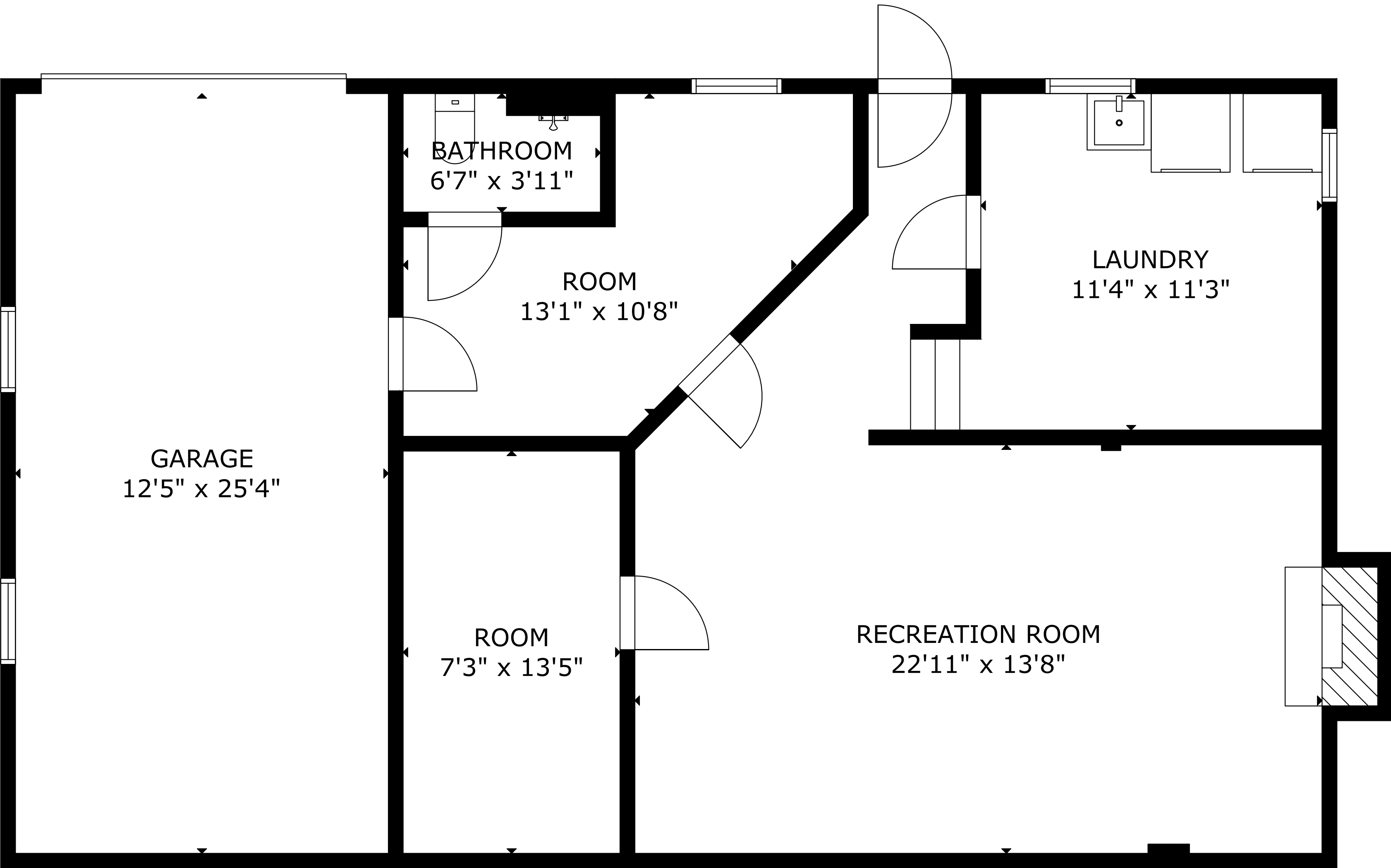
LOWER FLOOR
