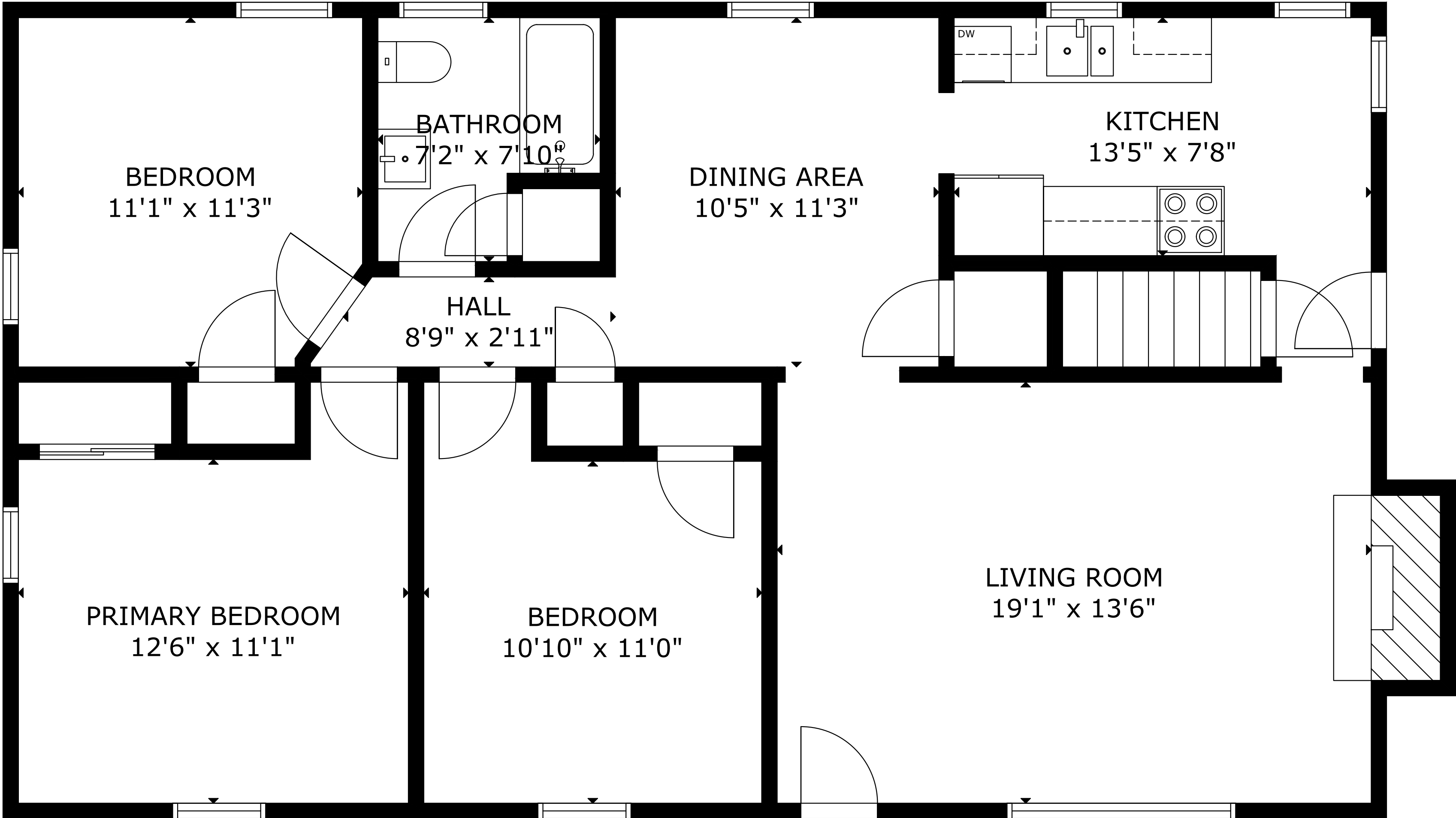
MAIN FLOOR
