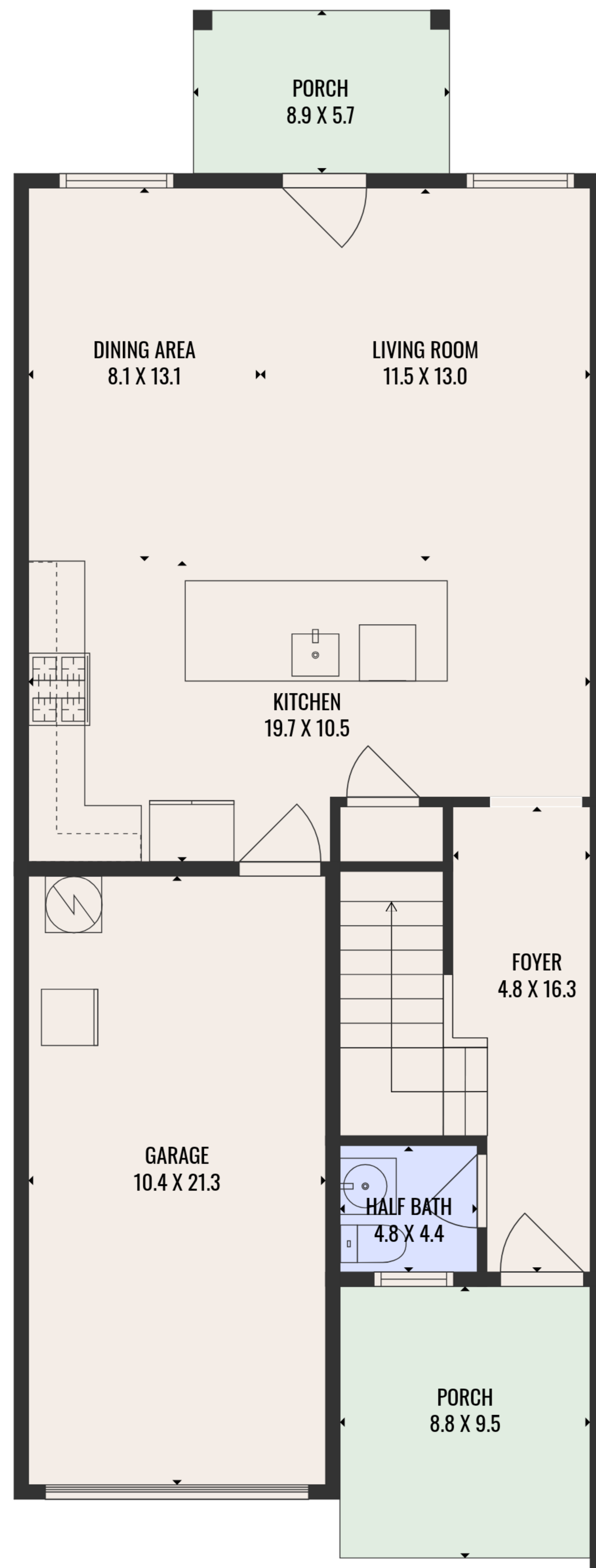
1ST FLOOR
